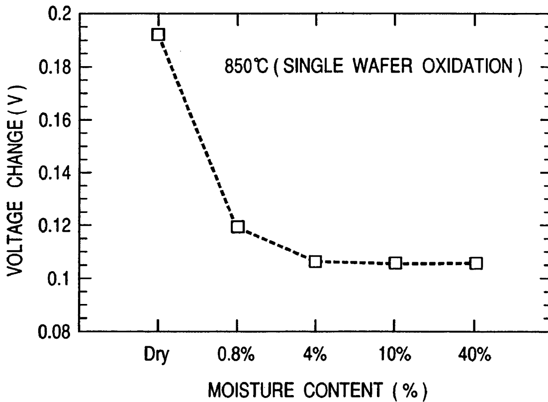
OXIDATION CONDITION DEPENDENCY OF VOLTAGE CHANGE
