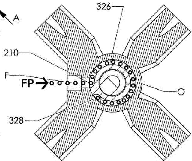
SECTION B-B FIG. 5D
