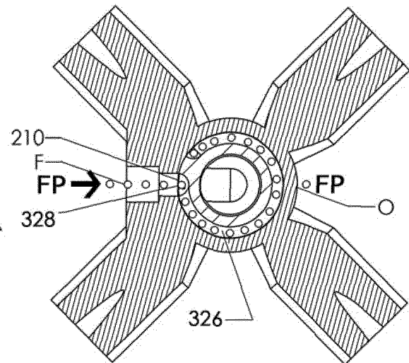
SECTION B-B FIG. 8D
