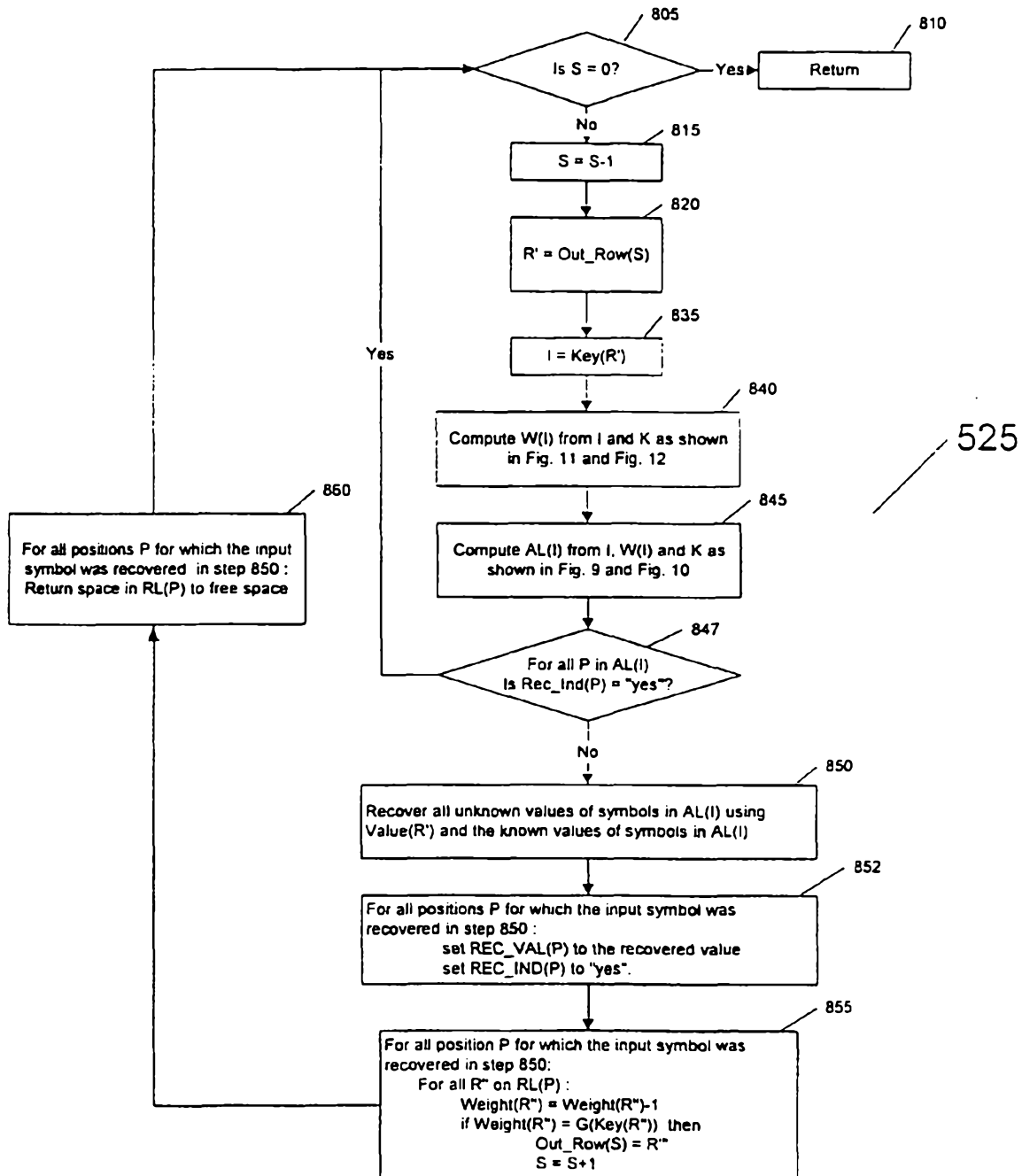
Recovery Processor Flow Chart Figure 8(a)
