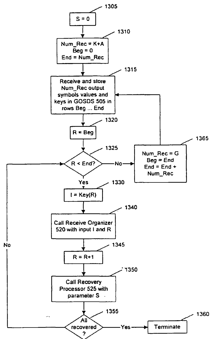
Lazy Decoder Figure 13
