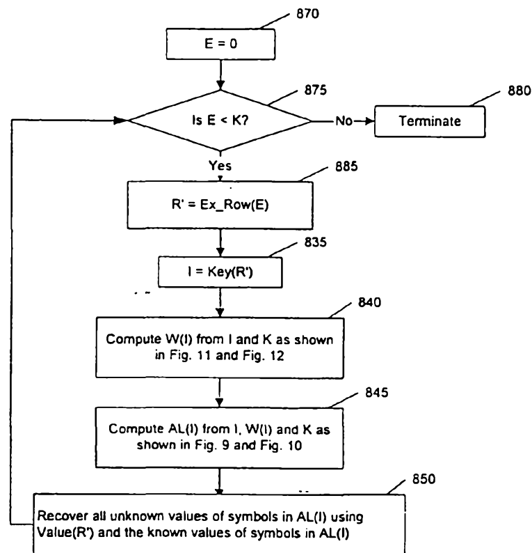
Process Execution Schedule Figure 8(c)
