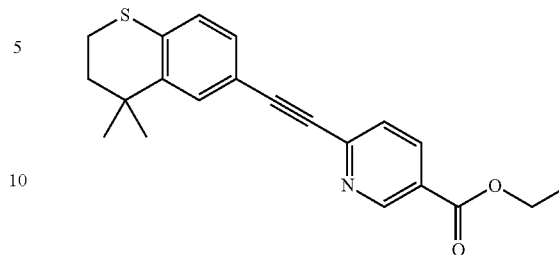
AGN 190168 (Tazarotene)
