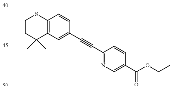
AGN 190168 (Tazarotene)
