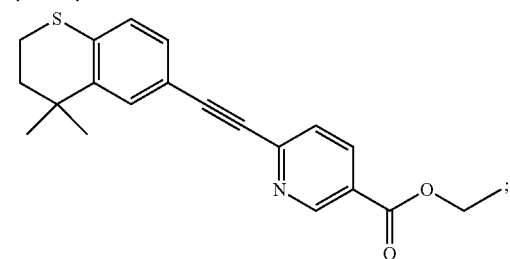
AGN 190168 (Tazarotene)
