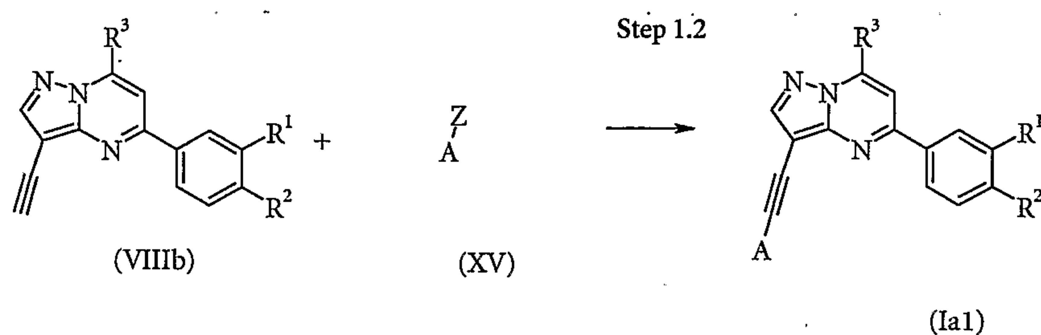
Scheme 2
