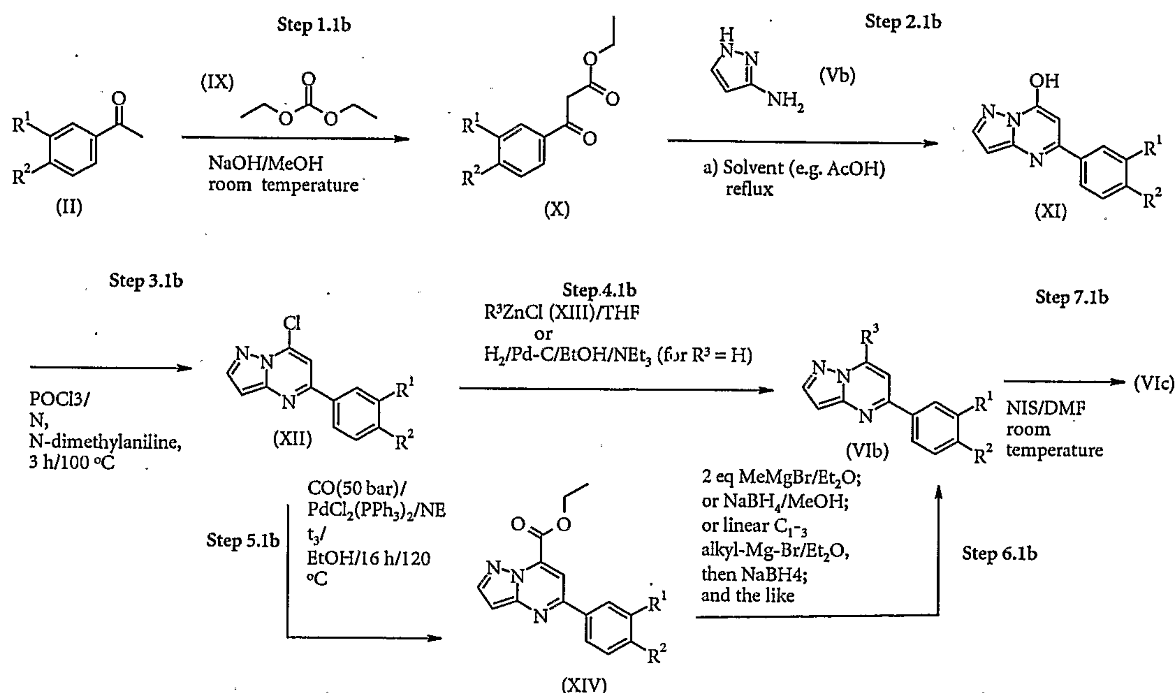
Scheme 1b
