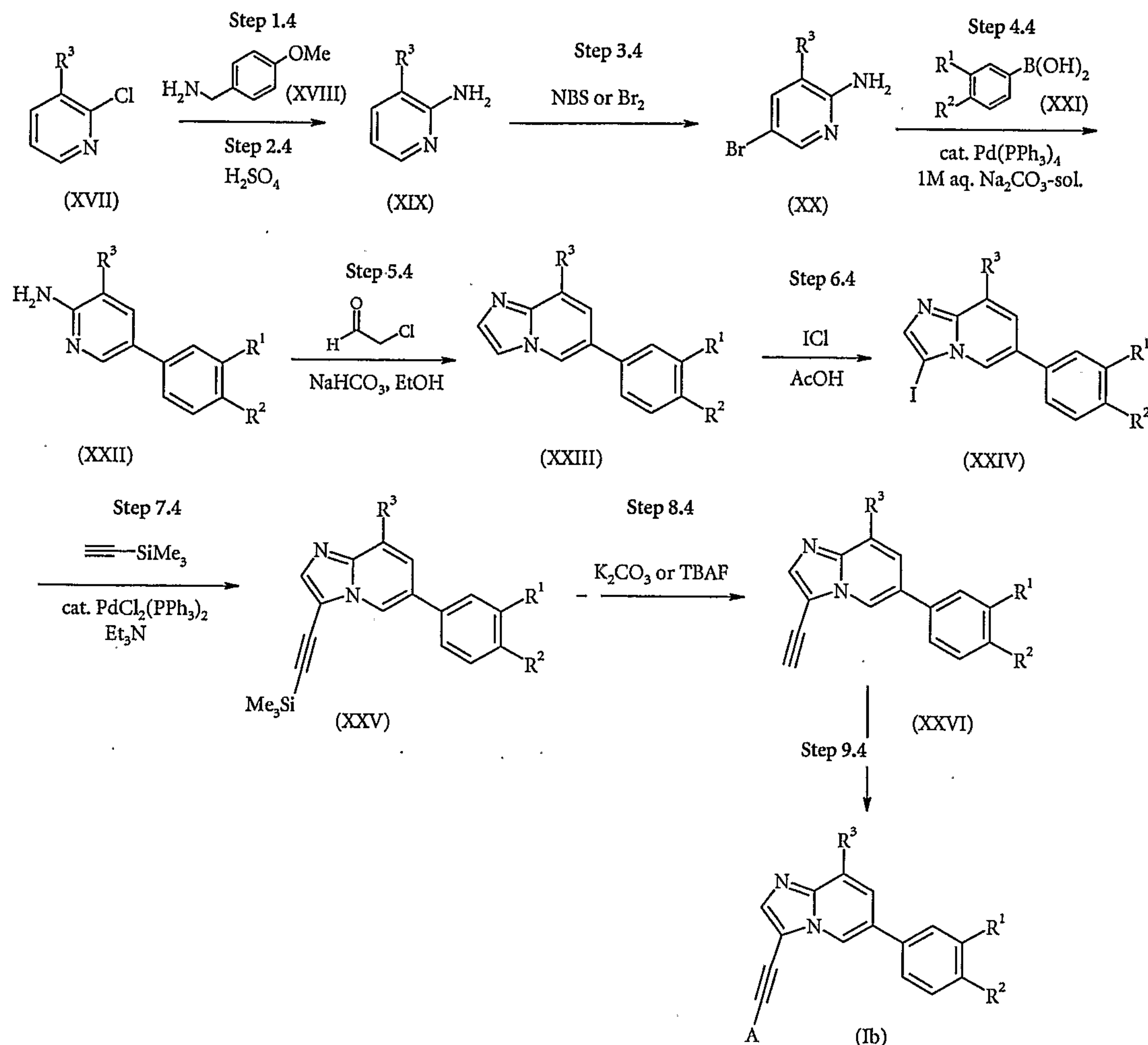
Scheme 4
