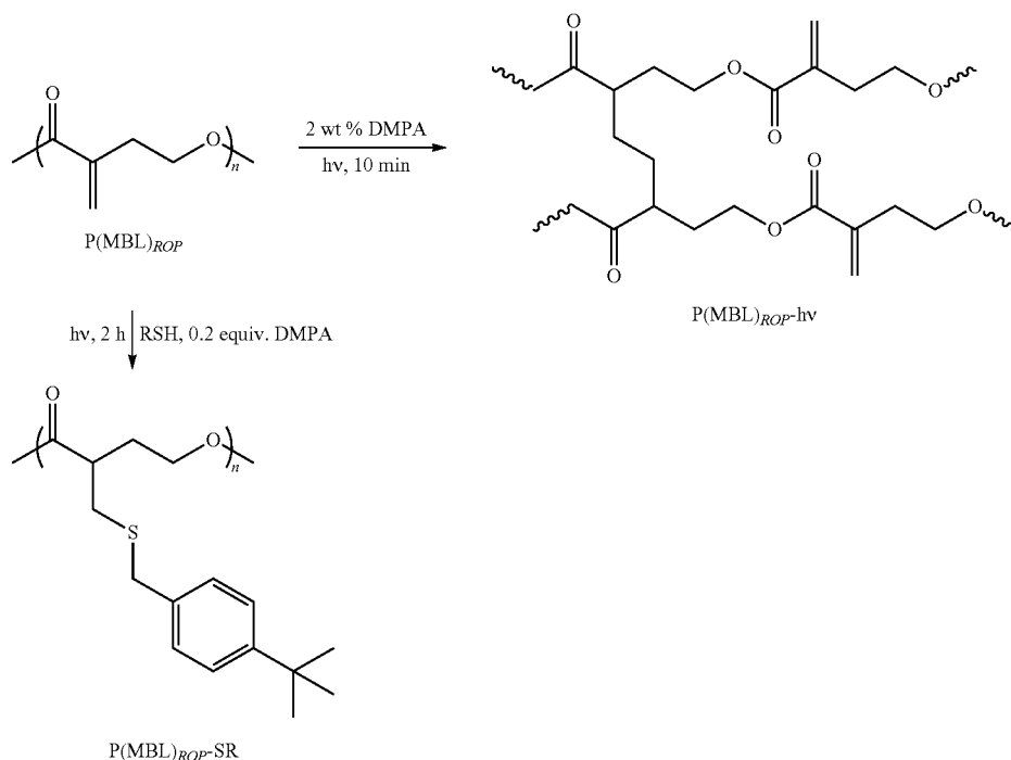
Scheme Z3. Post-functionalization of \text{P}(\text{MBL})_{ROP} via photocuring and the thiol-ene click reaction.
