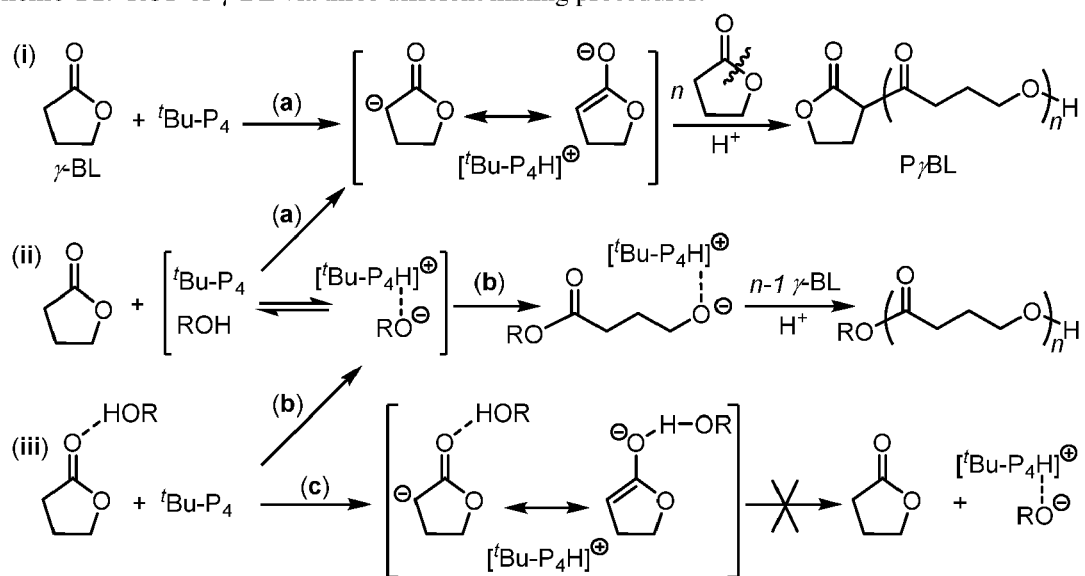
Scheme Y1. ROP of \gamma -BL via three different mixing procedures.
