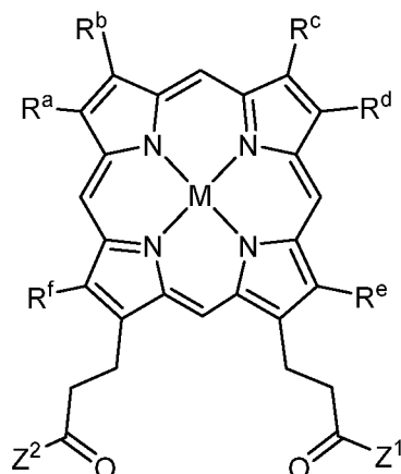
Formula I-B1
