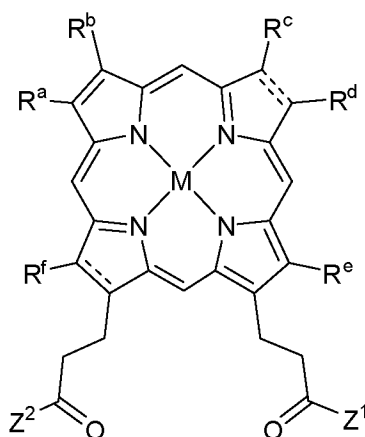
Formula I
