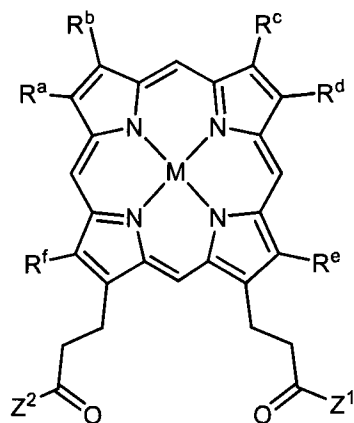
Formula I-B1
