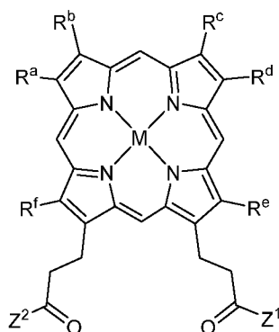
Formula I-B1
