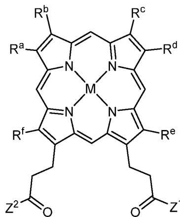
Formula I-B1
