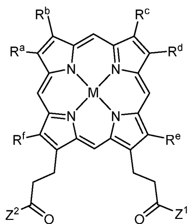
Formula I-B1
