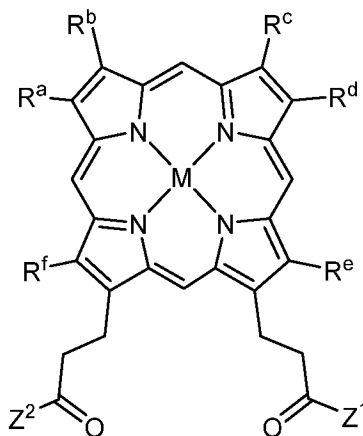
Formula I-B1
