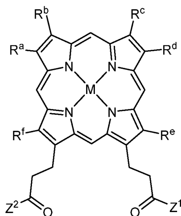
Formula I-B1
