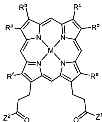
Formula I-B1
