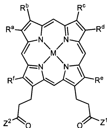
Formula I-B1
