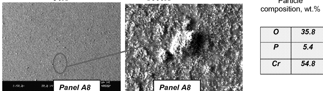
Fig.4. Coating system on Group A panel: SEM and EDS analysis
