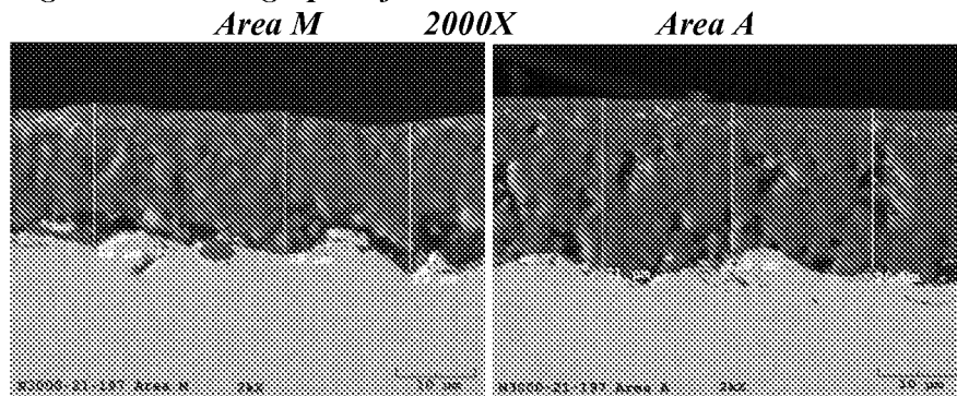
Fig.8. SEM micrographs of the coated Part 21-197 with measured thickness
