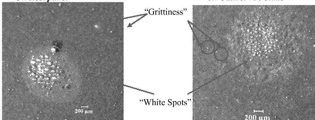
Fig.2 Typical defects of the prior art overlay system (Optical microscope 20X): On steel panel on Udimet 720 blade
