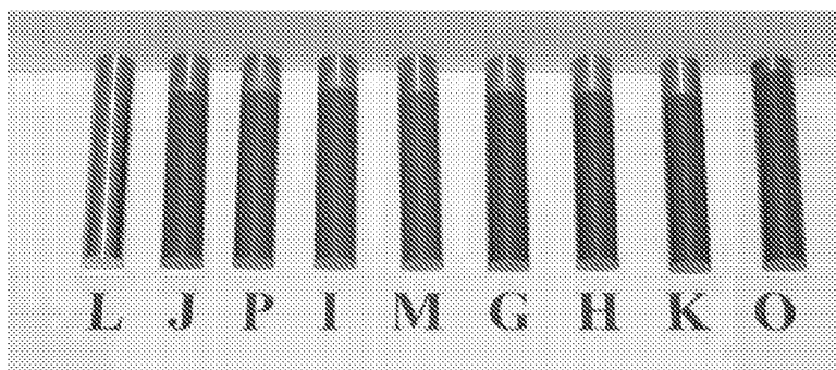
Fig.12. Multilayer Overlay System with different intermediate layer slurries on Udimet 720 pins: Before and after Hot Corrosion test
