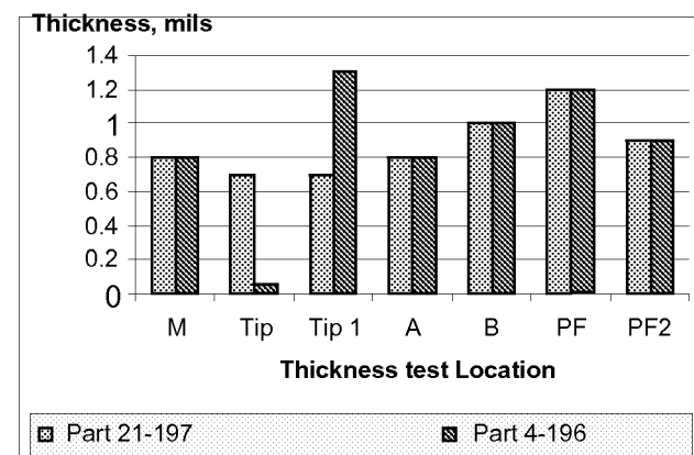
Fig.9. Coating system thickness in different areas on the parts
