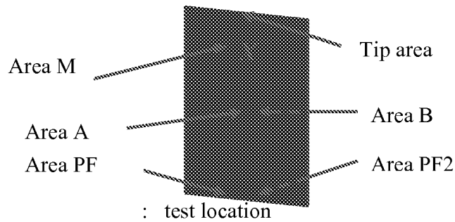
Fig.7. Diagram of a coated superalloy part showing thickness measurement locations
