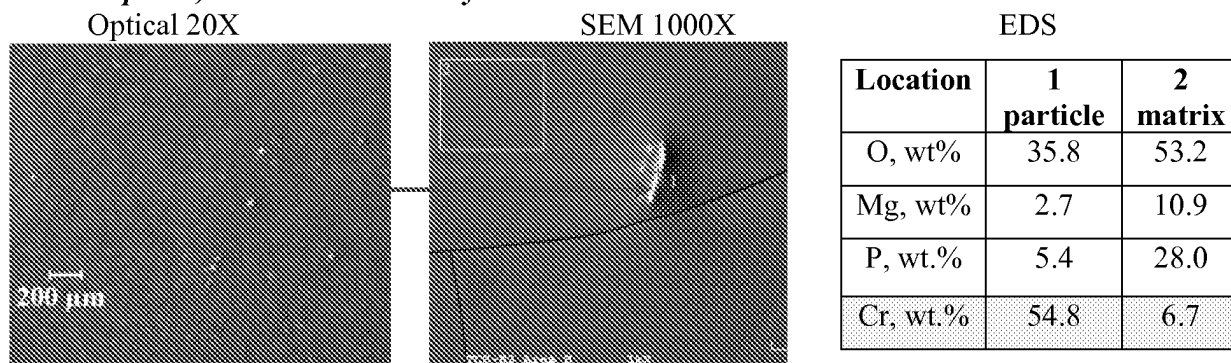
Fig.5 Multilayer overlay system of the prior art on steel panel: Optical, SEM and EDS analysis
