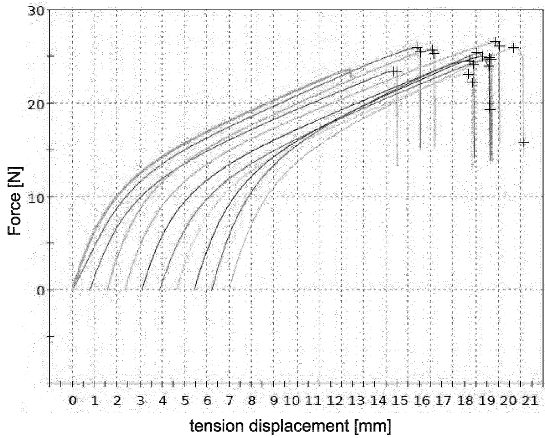
T2 strain/deformation profiles
