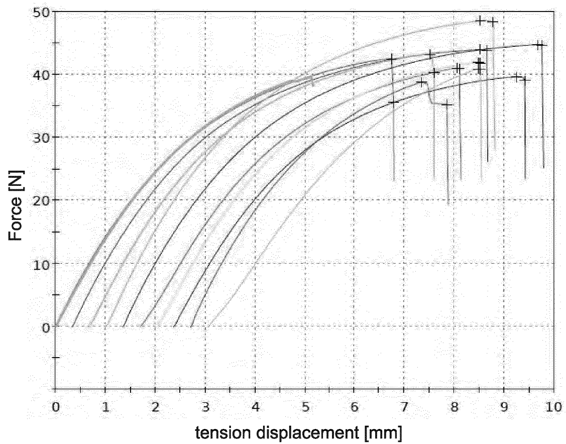
T3 strain/deformation profiles
