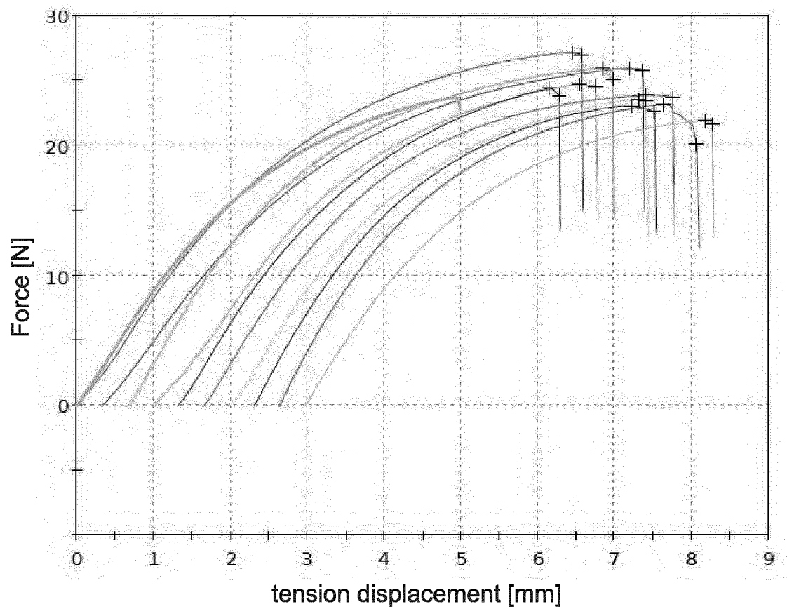
T4 strain/deformation profiles
