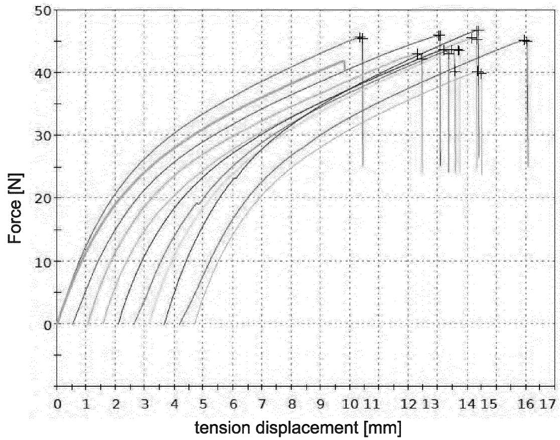
T6 strain/deformation profiles
