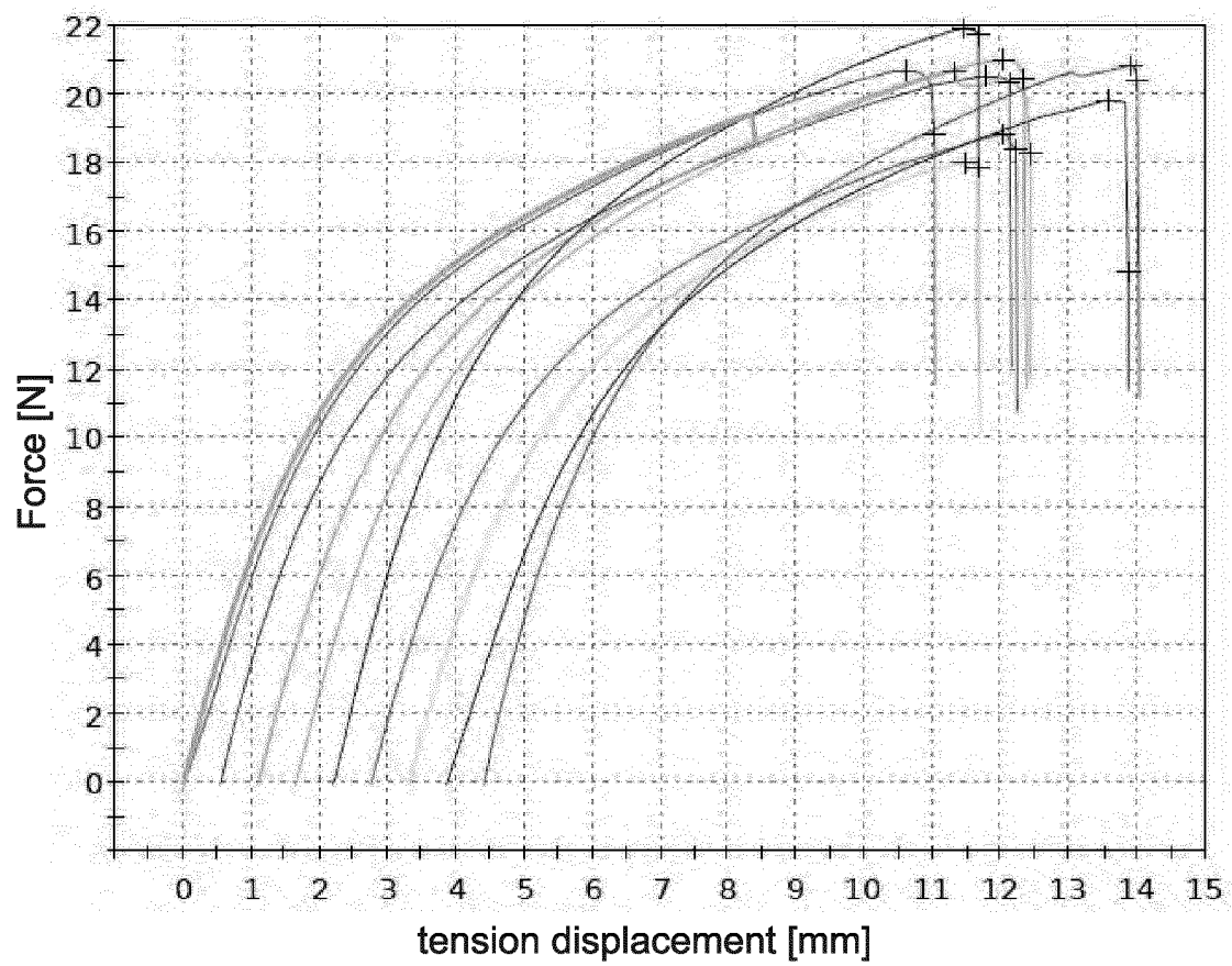
T1 strain/deformation profiles
