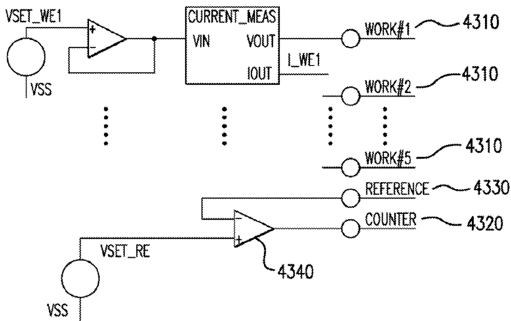
POTENTIOSTAT CONFIGURATION
