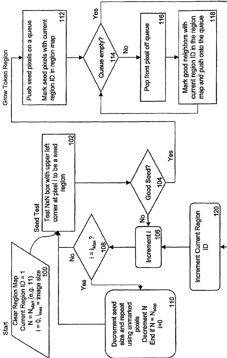
Figure 3A: Identifying Token Regions in an Image
