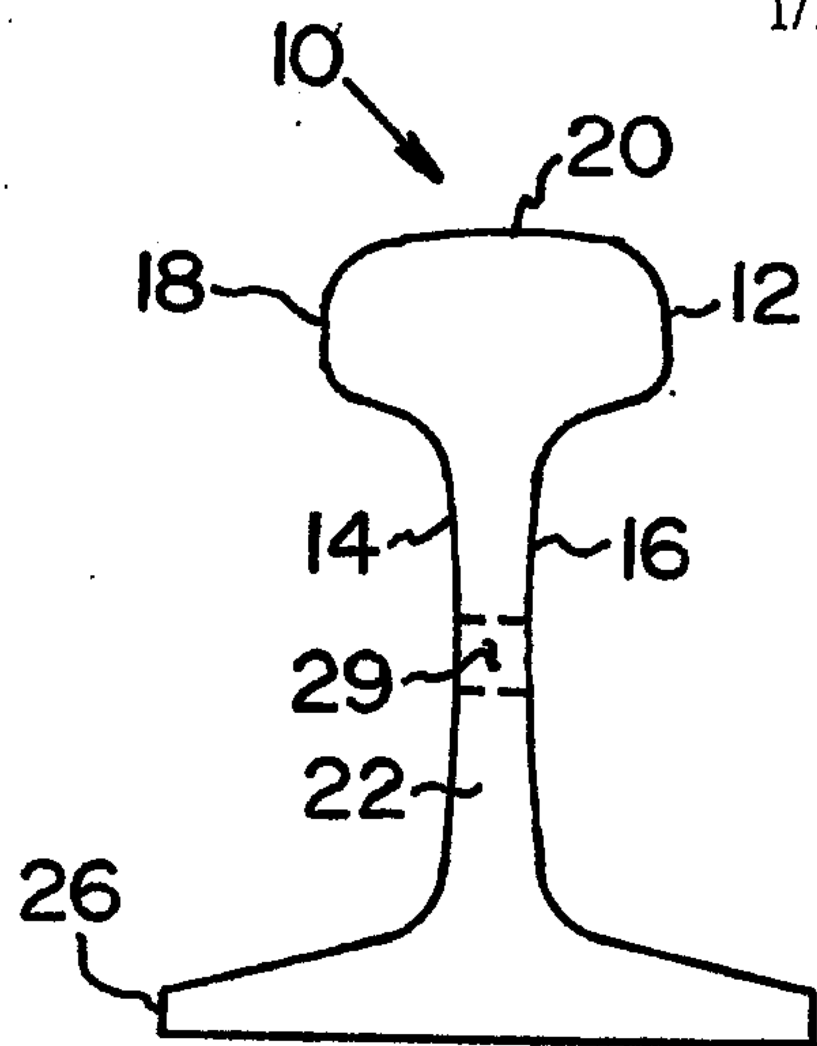
FIG. 1 (PRIOR ART)
