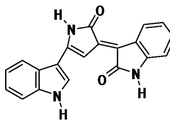
Deoxyviolacein (3)
