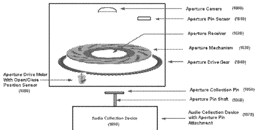
Drone ACD Deploy and Retrieve Mechanism
