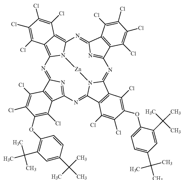
[Chemical Formula 10]
