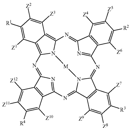
[Chemical Formula 1]
