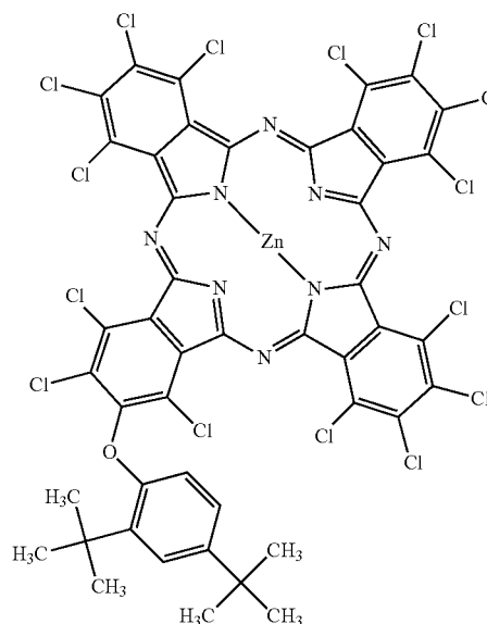
[Chemical Formula 11]
