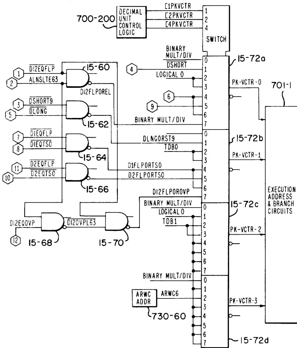
VECTOR BRANCH LOGIC FIG. 8 SHEET 2 OF 2
