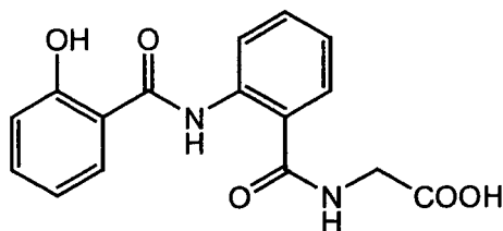
(compound 10)
