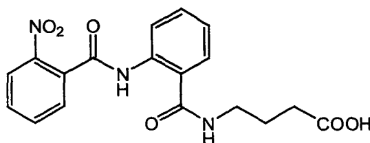
(compound 8)
