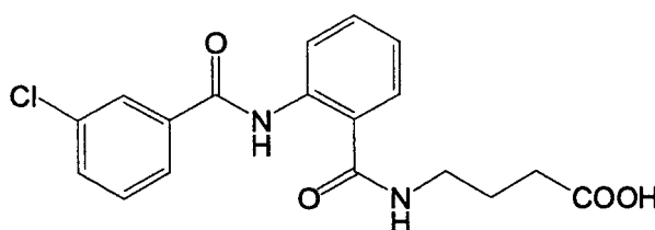
(compound 22)
