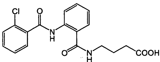
(compound 20)
