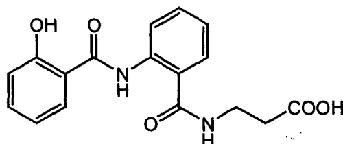
(compound 9)
