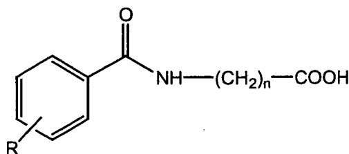
Structure B
