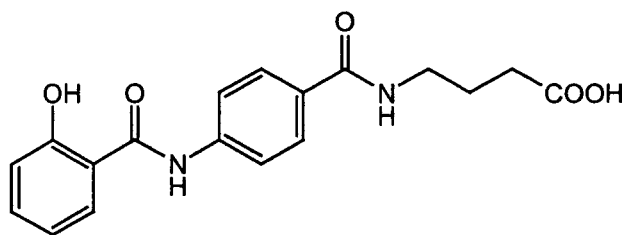
(compound 1)
