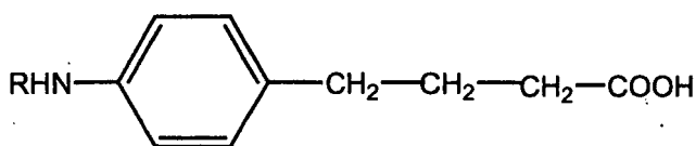
Structure A
