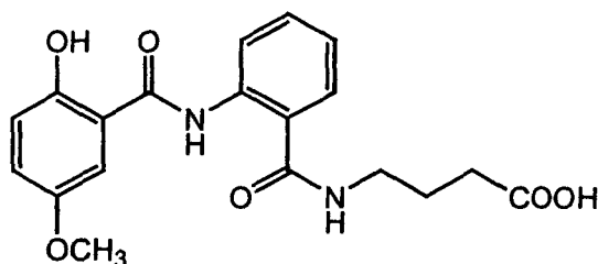
(compound 14)
