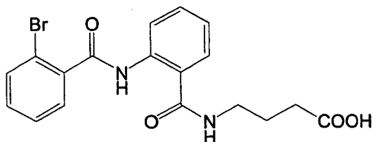
(compound 21)
