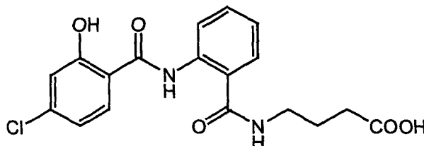
(compound 18)
