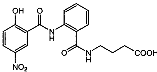
(compound 12)
