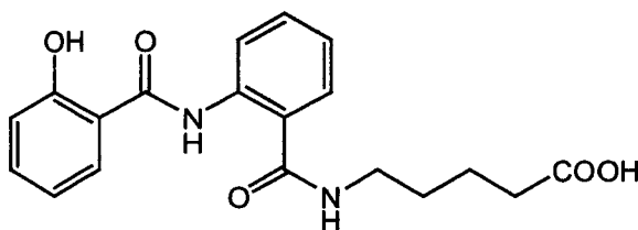
(compound 5)
