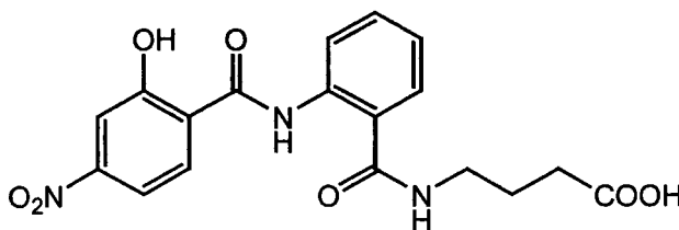
(compound 11)
