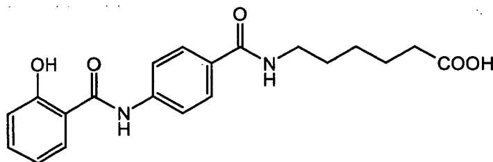
(compound 2)
