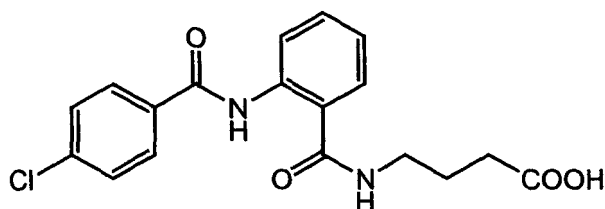
(compound 17)
