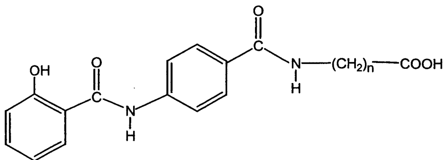
Structure C
