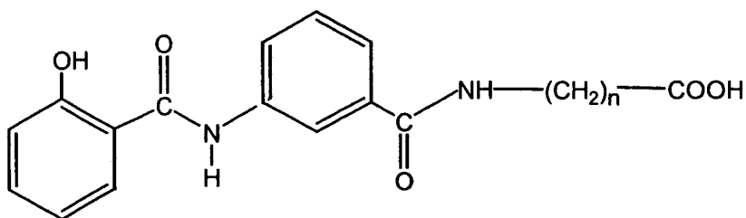
Structure D
