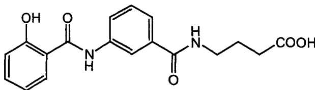
(compound 3)
