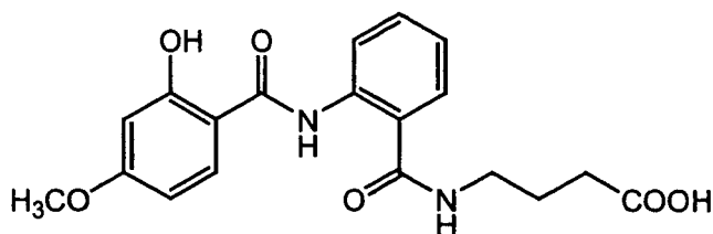
(compound 13)
