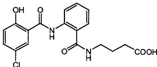
(compound 19)
