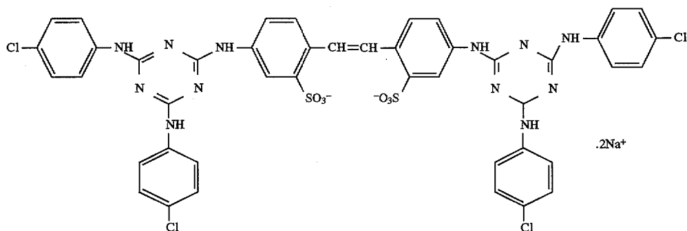
supersensitizer cpd 2
