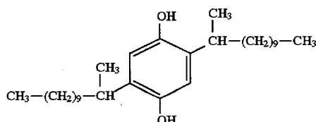
scavenger cpd 3
