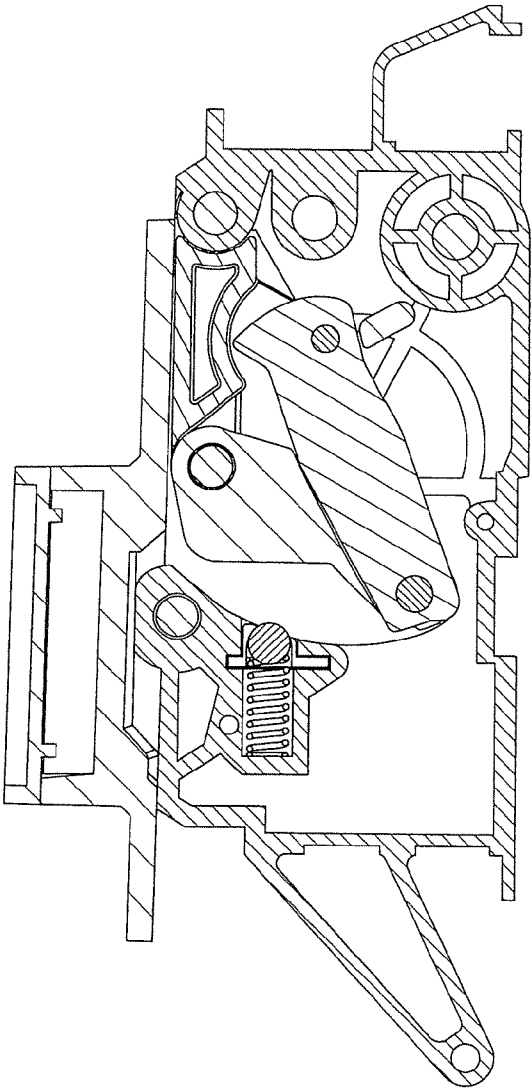
SECTION C-C
