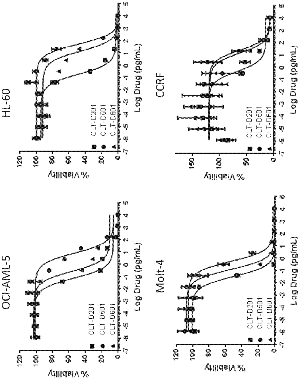
FIG. 10 IQB Payloads – Cytotoxicity on Leukemia Cell lines
