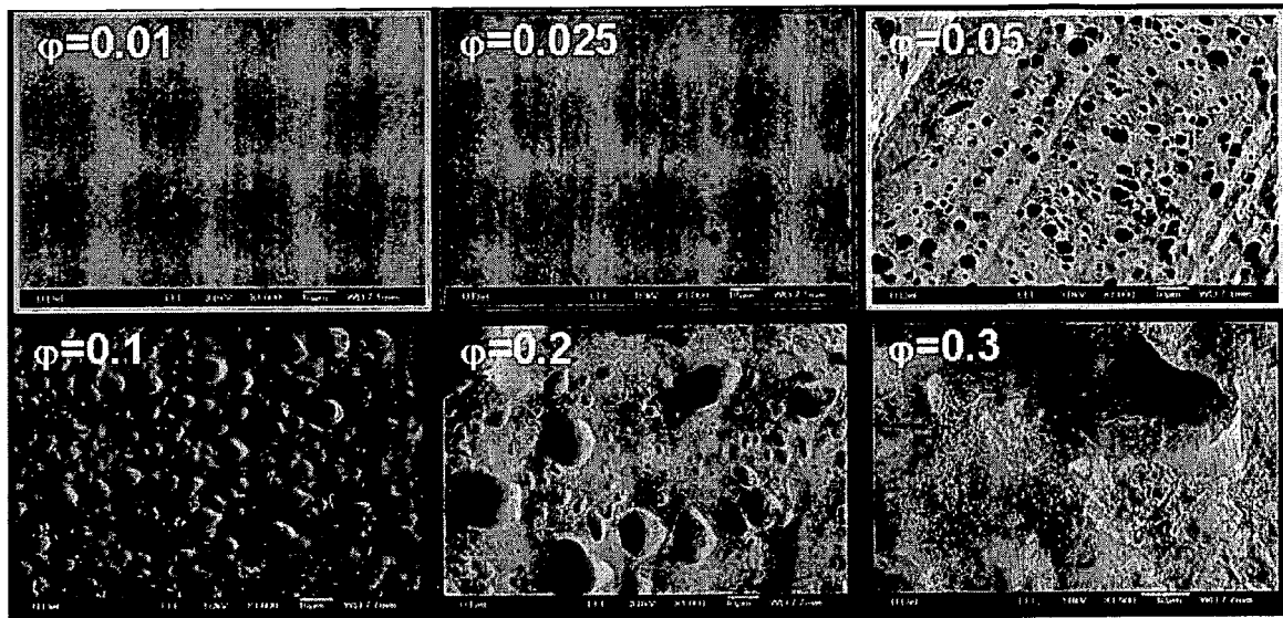
Figure 9. SEM images of STF-PO blend morphology. STF inclusions are evident as holes or particle filled voids, which is a consequence of sample preparation and PEG loss in the electron beam.
