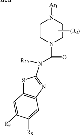
Piperazine Compounds
