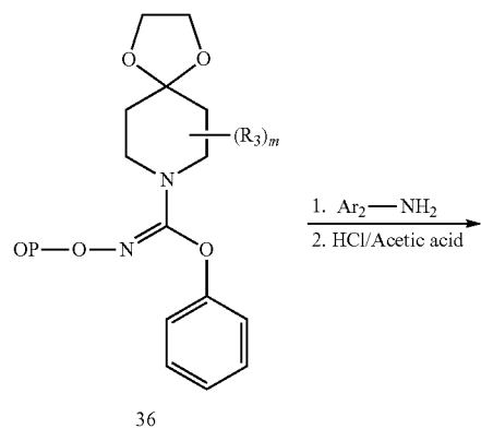
Scheme 2.8
