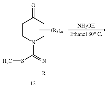
Scheme 1.7
