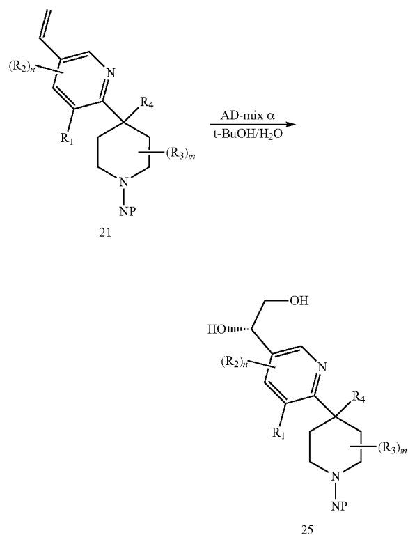
Scheme 1.14
