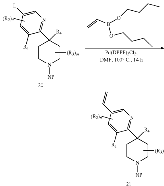
Scheme 1.12
