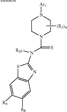
Piperazine Compounds
