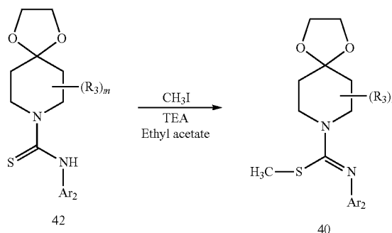
Scheme 2.10
