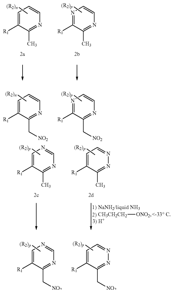
Scheme 1.11
