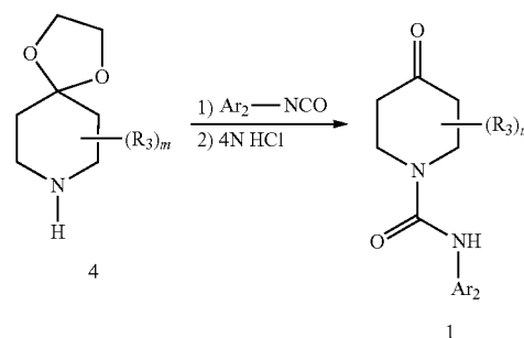
Scheme 1.2
