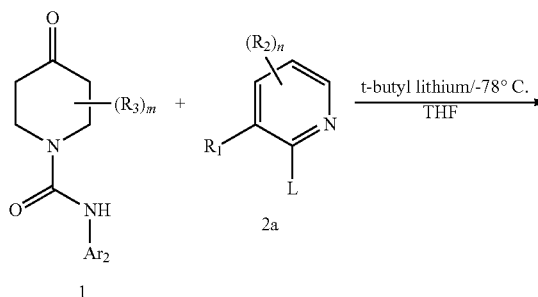
Scheme 1.1
