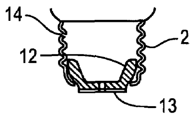
FIG. 3 PRIOR ART
