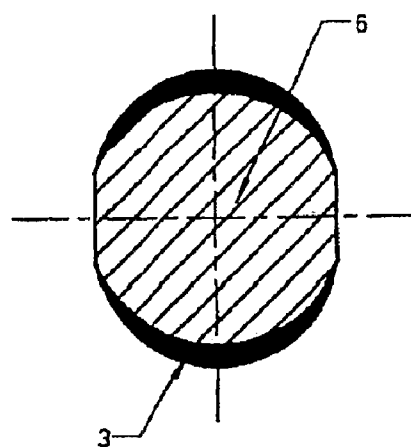
SECTION A - A FIGURE 5
