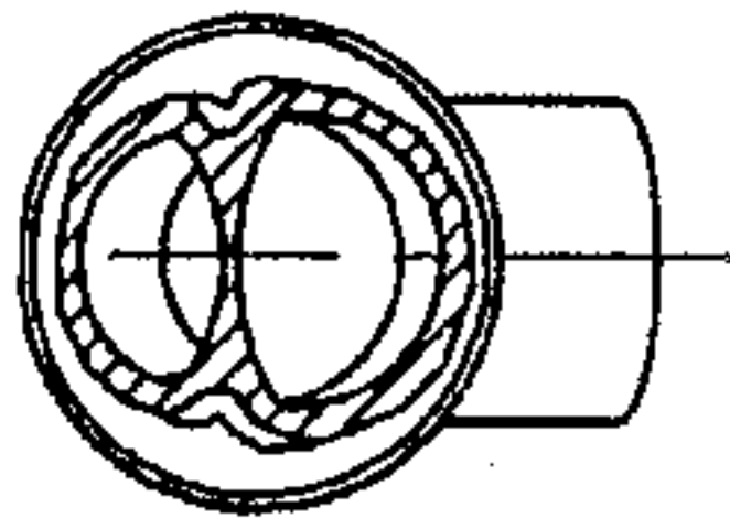
SECTION 18-18 FIG. 4j
