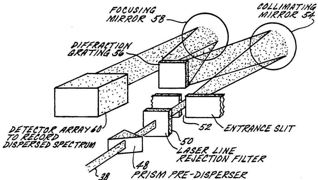
SPECTROGRAPH WITH LINE FILTER ON ITS INPUT
