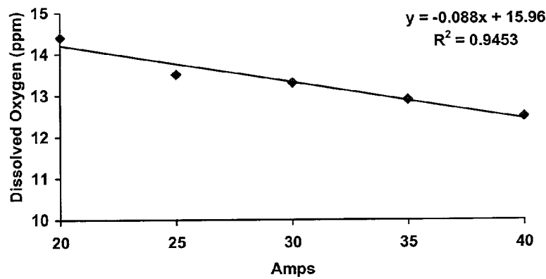
Figure 1 Effect of increasing water flow rate (current) on dissolved oxygen content
