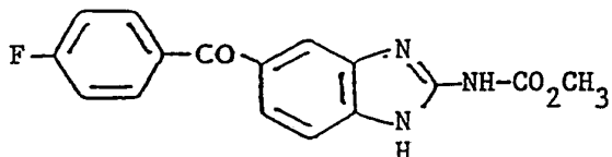
Flubendazole
