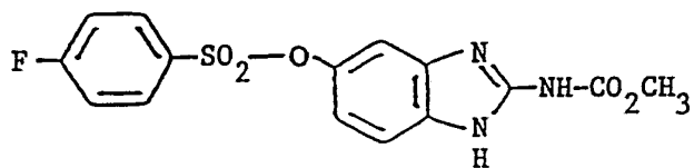
Luxobendazole
