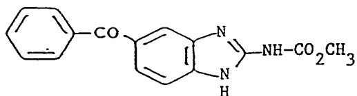
Mebendazole
