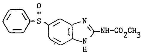
Oxfendazole
