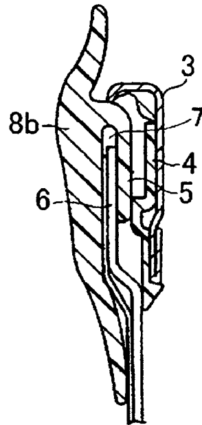
FIG. 4 [ Prior art ]
