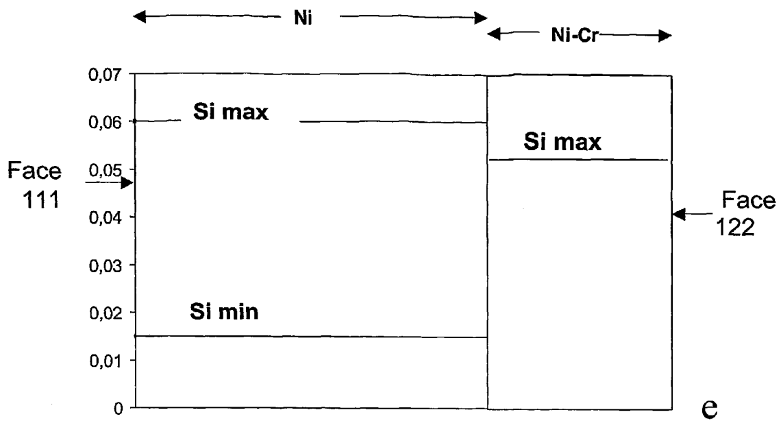
Fig.5 – PRIOR ART
