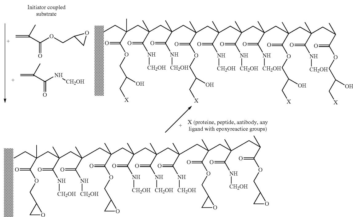
Reaction scheme 3
