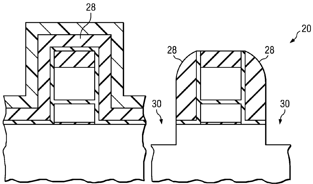
FIG. 2c (PRIOR ART)
