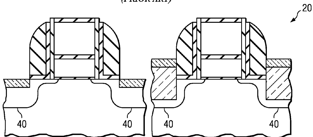
FIG. 2i (PRIOR ART)
