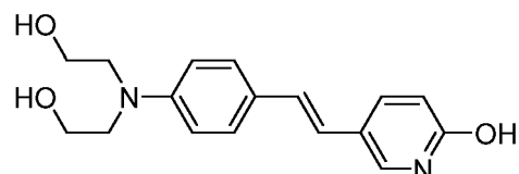
Compound vi
