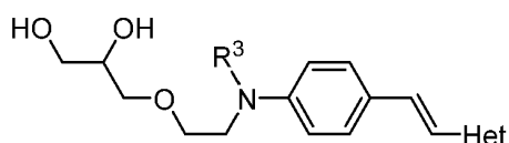
Compounds B
