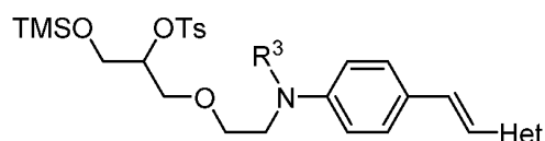
Compounds F
