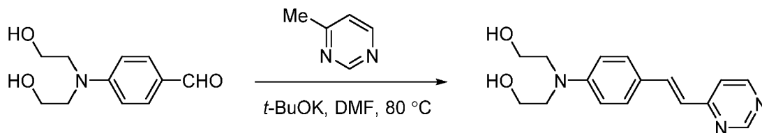
Compound iii
