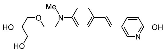
Compound vii
