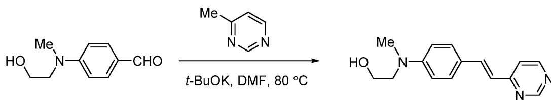
Compound ii
