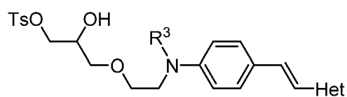
Compounds C
