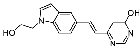
Compound xii
