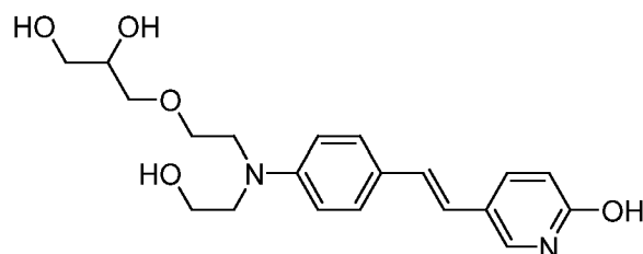
Compound ix
