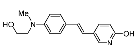
Compound v
