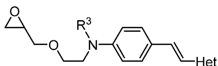
Compounds D
