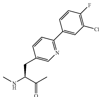
4-[(3'-Chloro-4'-fluoro)phenyl]- 3-pyridylalanine
