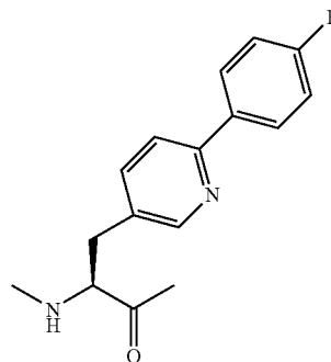
4-(4'-Fluorophenyl)- 3-pyridylalanine
