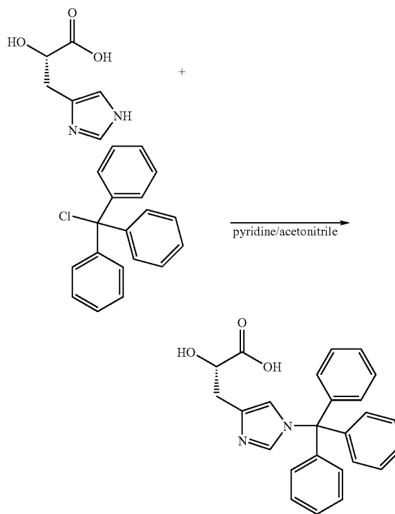
SCHEME 22
