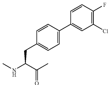
Bip(3'-Cl-4'-F)
