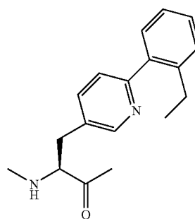
4-(2'-Ethylphenyl)-3-pyridylalanine
