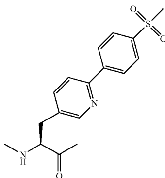
4-(4'-methanesulfonylphenyl)- 3-pyridylalanine
