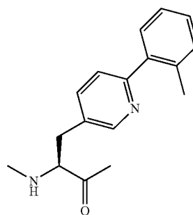
4-(2'-Methylphenyl)-3-pyridylalanine
