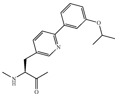
4-(3'-Isopropoxyphenyl)- 3-pyridylalanine
