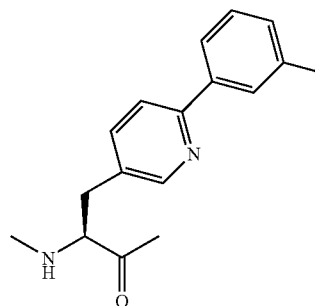
4-(3'-methylphenyl)- 3-pyridylalanine
