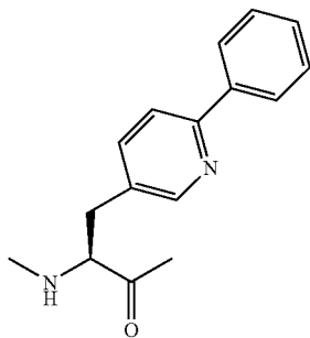
4-phenyl-3-pyridylalanine
