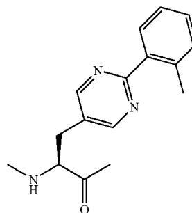
4-(2'-Methylphenyl)- 3,5-pyrimidylalanine
