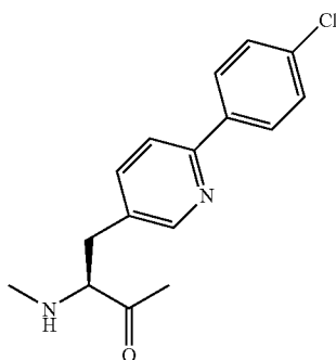
4-(4'-Chlorophenyl)- 3-pyridylalanine
