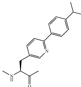
4-(4'-Isopropylphenyl)- 3-pyridylalanine
