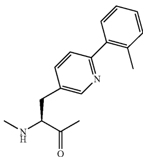
4-(2'-Methylphenyl)- 3-pyridylalanine
