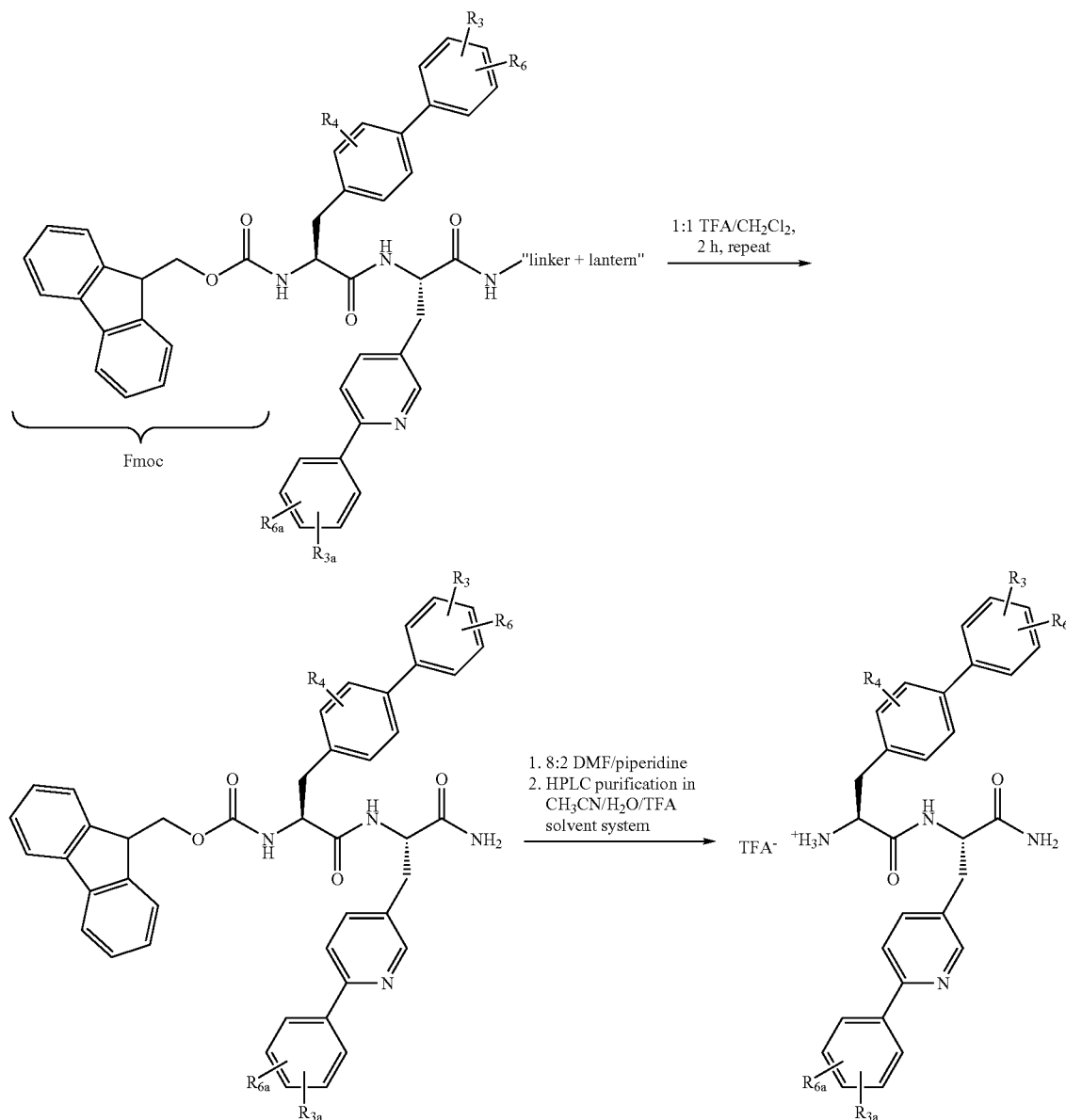
SCHEME 8
