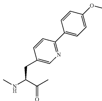
4-(4'-Methoxyphenyl)- 3-pyridylalanine
