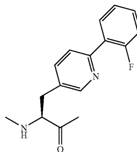
4-(2'-fluorophenyl)- 3-pyridylalanine
