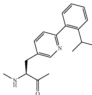
4-(2'-Isopropylphenyl)- 3-pyridylalanine
