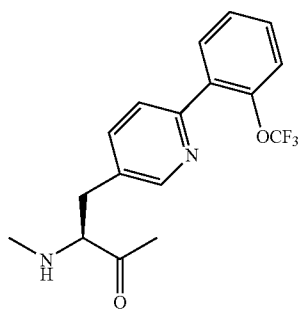
4-(2'-Trifluoromethoxyphenyl)- 3-pyridylalanine
