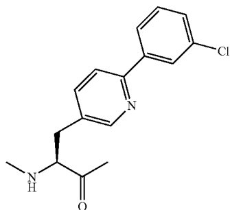
4-(3'-Chlorophenyl)-3- pyridylalanine
