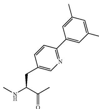
4-(3',5'-dimethylphenyl)- 3-pyridylalanine
