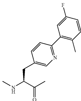
4-[(2'-Methyl-5'-fluoro)phenyl]- 3-pyridylalanine
