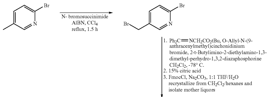
SCHEME 14
