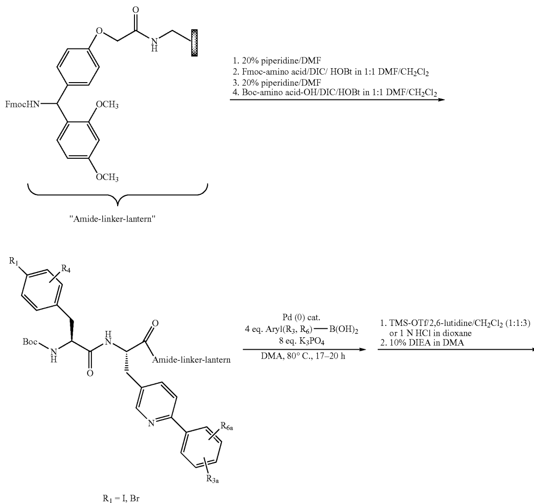
SCHEME 4
