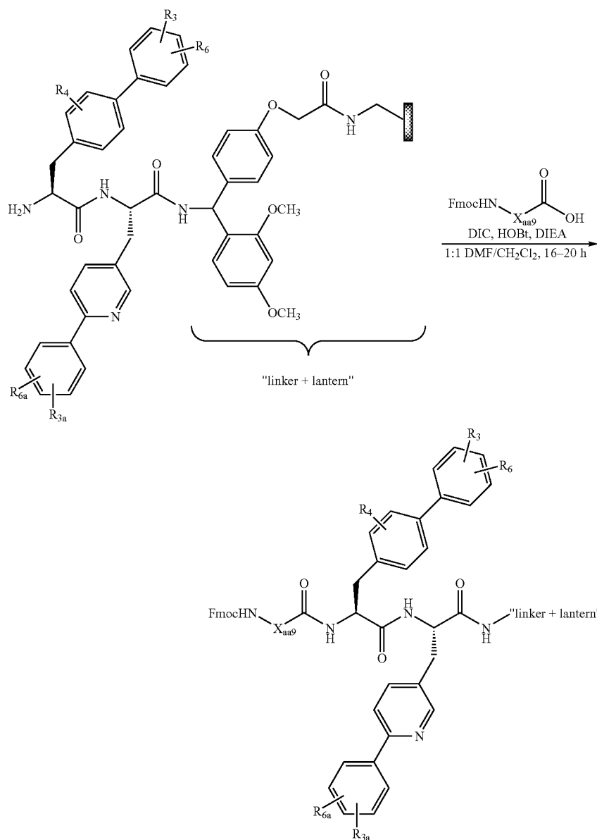
SCHEME 6
