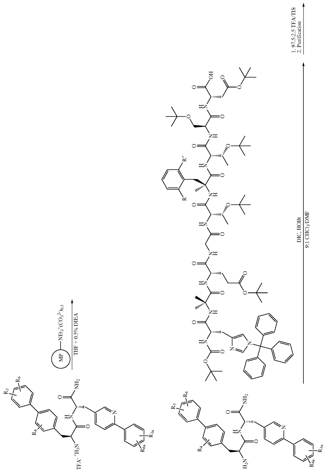
SCHEME 10
