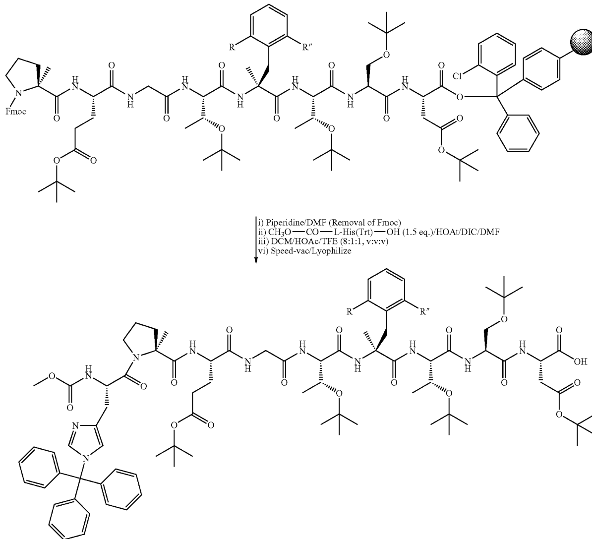
SCHEME 9B
