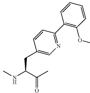
4-(2'-Methoxyphenyl)- 3-pyridylalanine
