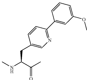
4-(3'-Methoxyphenyl)- 3-pyridylalanine
