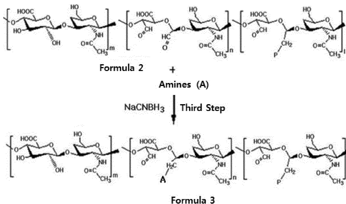
[Reaction scheme 2]
