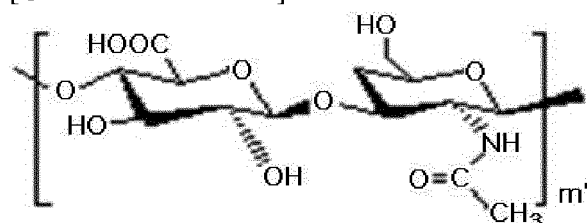
[Chemical formula 1]
