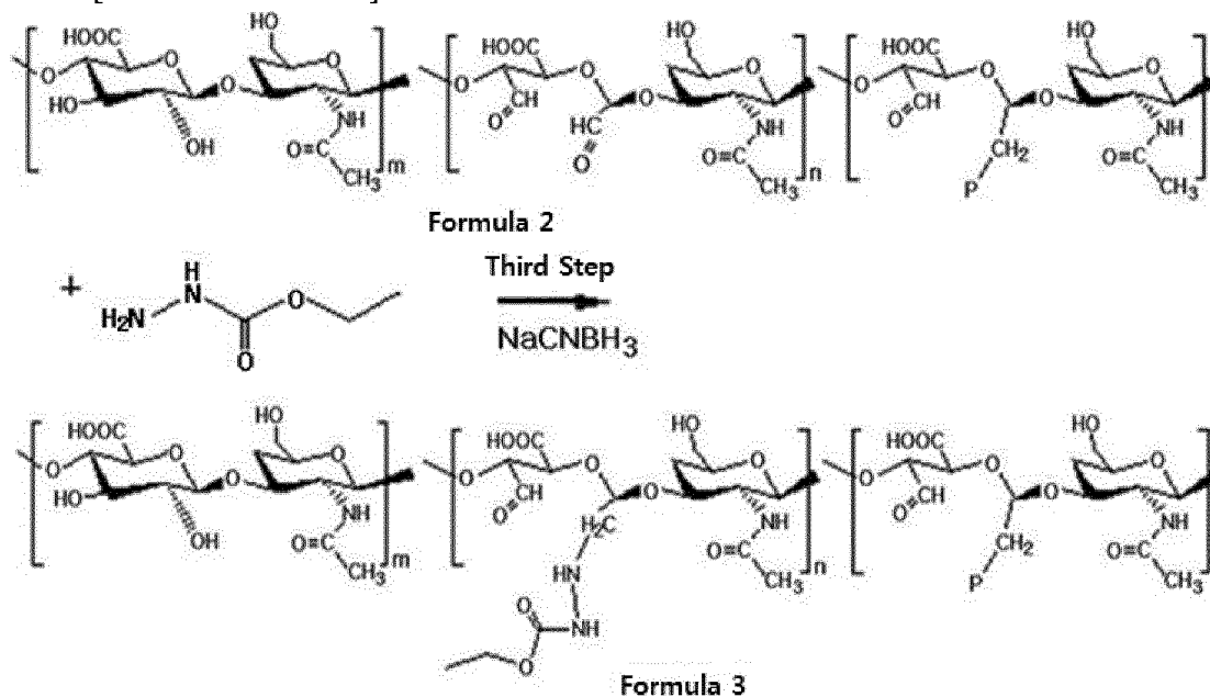
[Reaction scheme 3]
