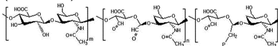
[Chemical formula 2]
