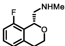
Compound 1; and
