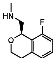
Compound 1.
