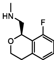
(Compound 1).
