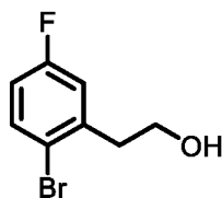
Compound 3.
