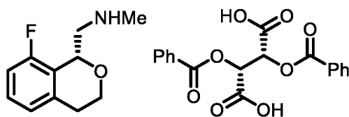
Compound 1 dibenzoyl-L-tartrate
