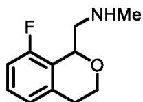
Racemic Compound 1,
