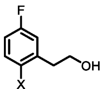
Formula III,
