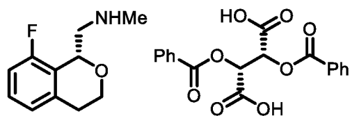
Compound 1 dibenzoyl-L-tartrate
