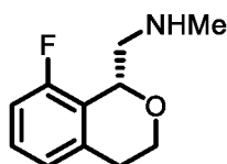
Compound 1,
