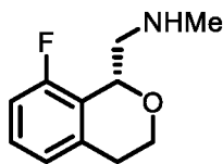
Compound 1
