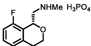
Compound 1 Phosphate
