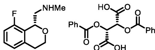
Compound 1 dibenzoyl-L-tartrate
