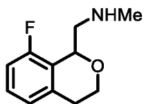
Racemic Compound 1;
