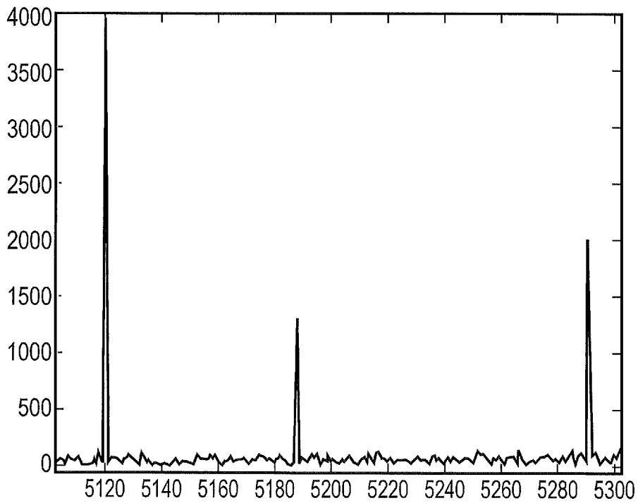
Matched filter output for multipath channel
