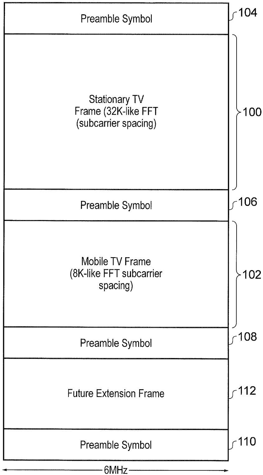
Framing concept for ATSC3-0
