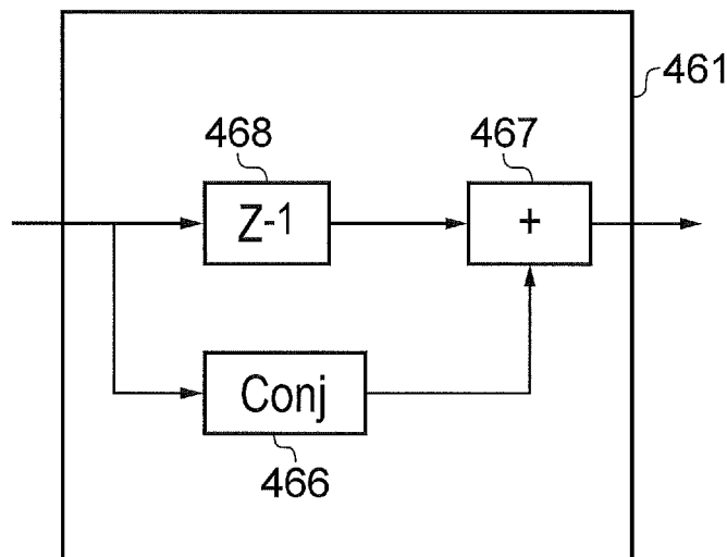
Differential Encoder
