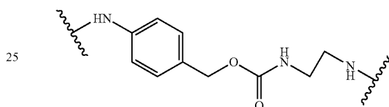
(MP, maleimidopropanoyl containing)
