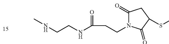
(MP, maleimidopropanoyl containing)
