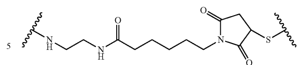
(MC, 6-maleimidocaproyl containing)
