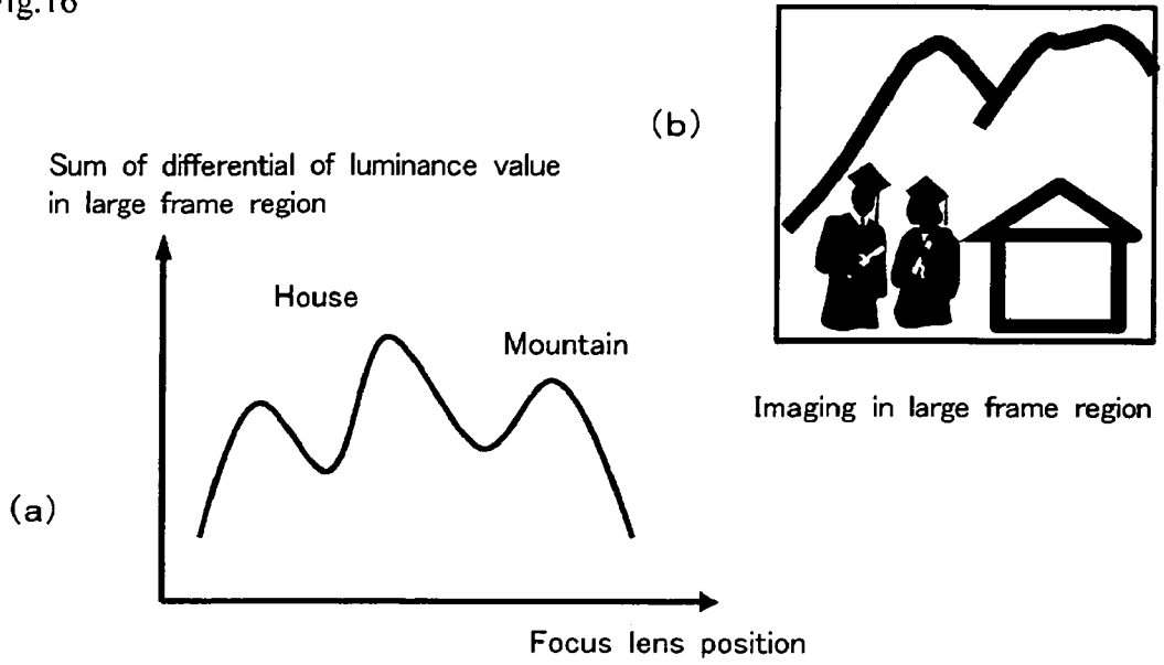
Correlation between focus lens position in large frame region and luminance value in large frame region
