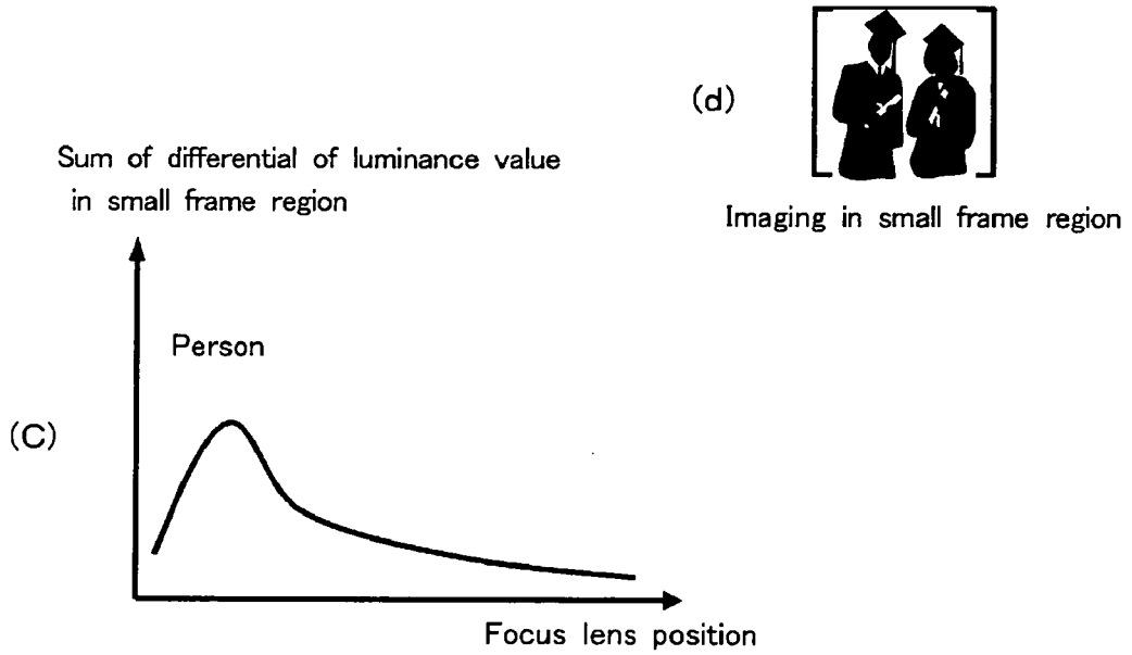
Correlation between focus lens position in small frame region and luminance value in large frame region
