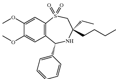
(3R, 5R)-3-butyl-3-ethyl-2, 3, 4, 5-tetrahydro-7, 8-dimethoxy-5-phenyl-1,4-benzothiazepine 1, 1-dioxide
