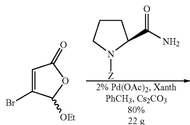
Scheme 2. Synthetic Examples
