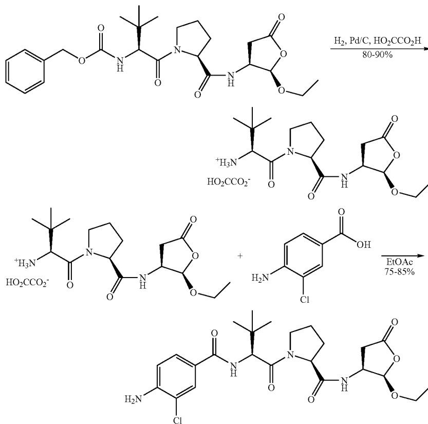
Scheme 3
