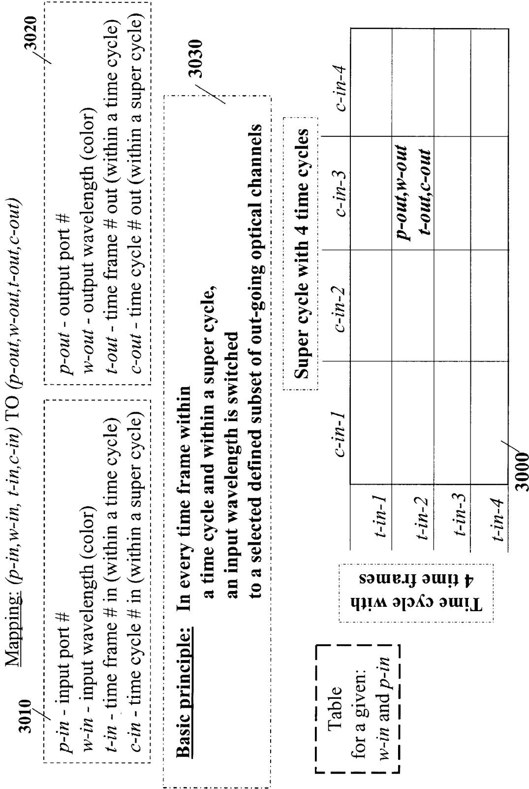
FIG. 30 Optical switching & forwarding of time frames
