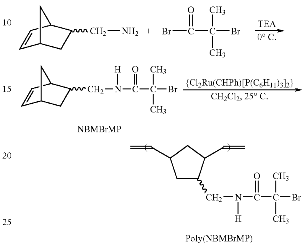
Scheme I. Synthesis and ring-opening metathesis polymerization of NBMBBrMPA
