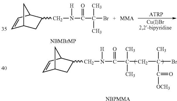
Scheme II. Preparation of macromonomer (NBPMMMA)
