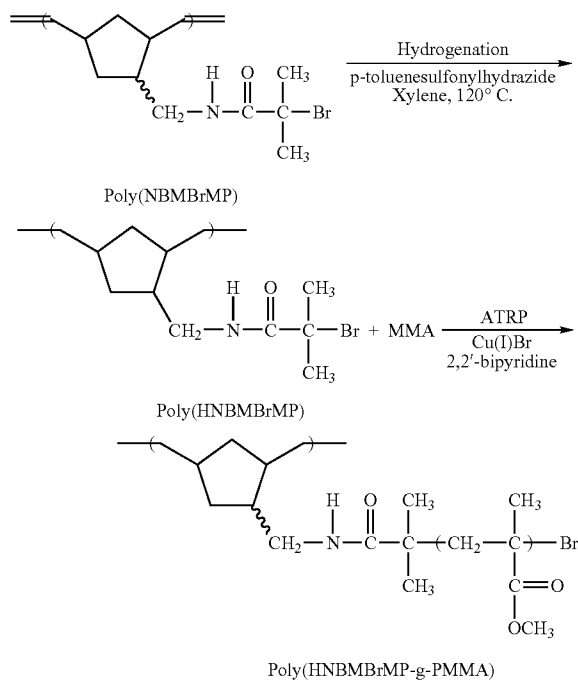
Scheme IV. Synthesis of poly(HNBMBrMPA) and poly(HNBMBrMPA-g-PMMA)
