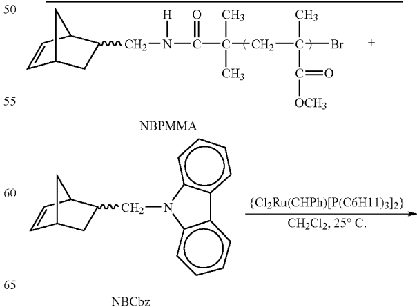
Scheme III. Ring-opening metathesis polymerization of NBCbz and NBPMMMA
