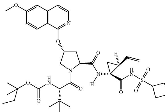
Compound 382
