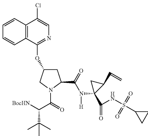
Compound 281
