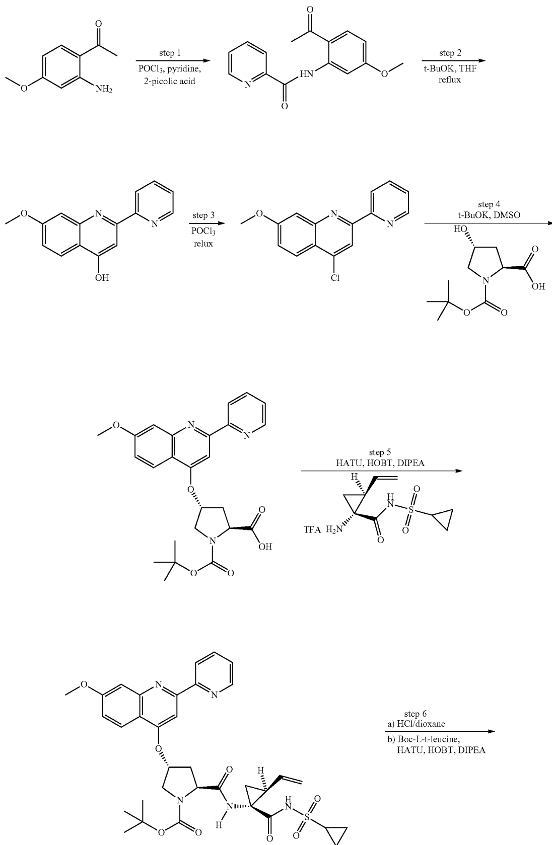
Scheme 1
