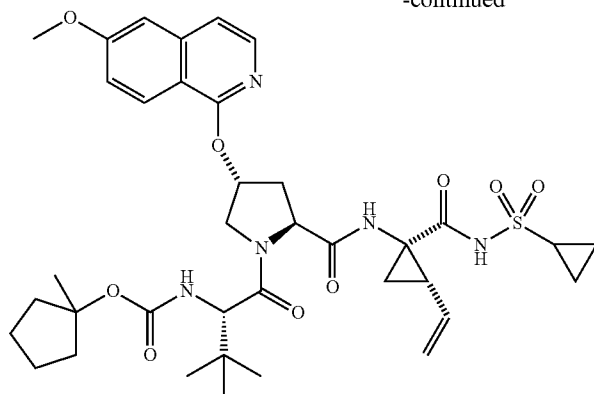
Compound 69
