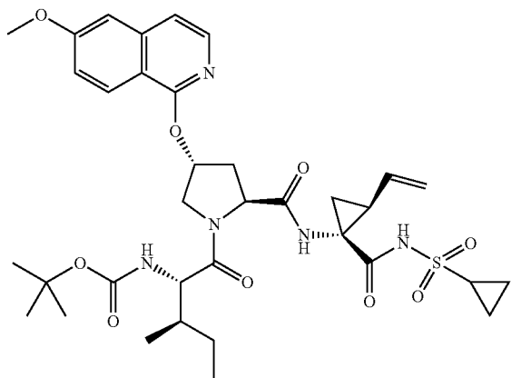
Compound 13
