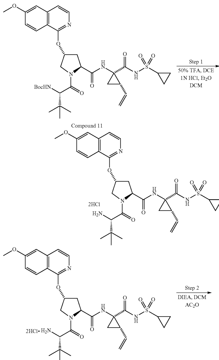
Scheme 1
