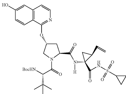
Compound 280 10
