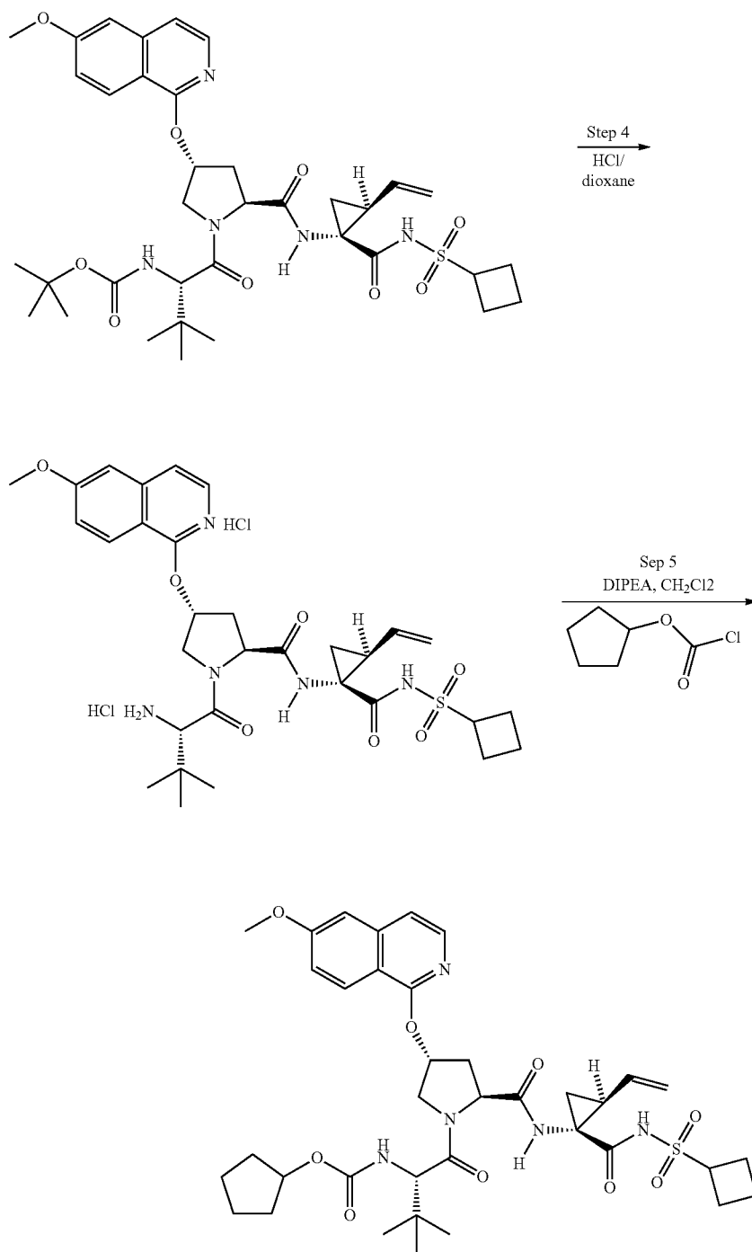
Compound 380
