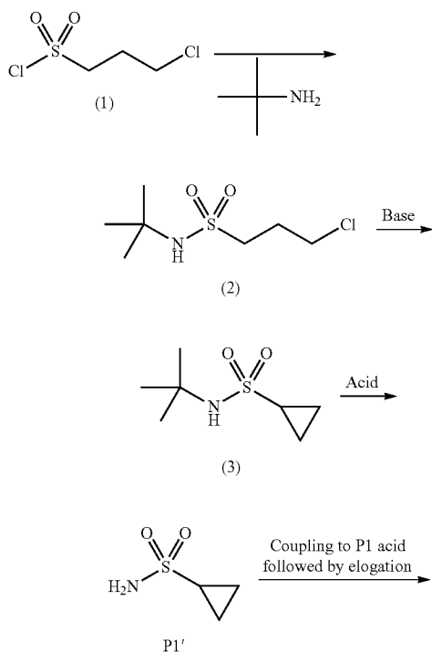
Scheme VII
