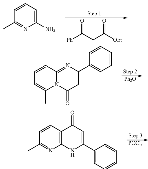
Scheme 1
