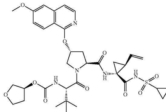
Compound 19
