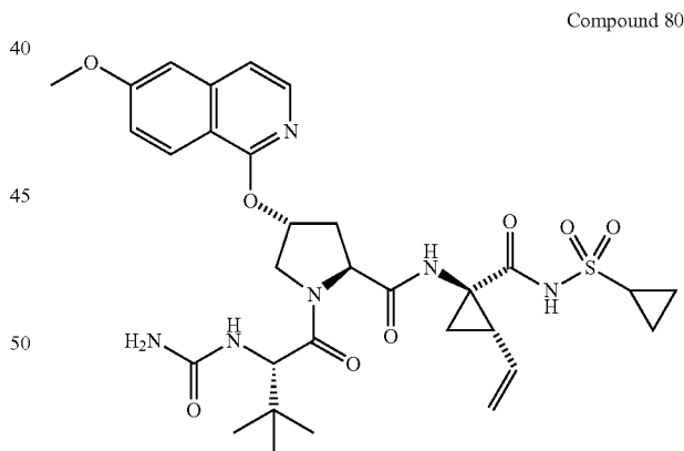
Compound 80
