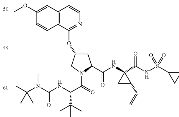
Compound 77
