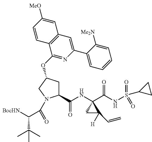
Compound 329
