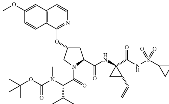
Compound 85
