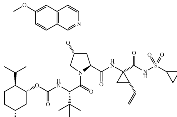
Compound 66
