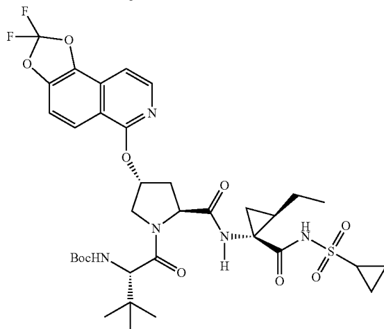
Compound 289
