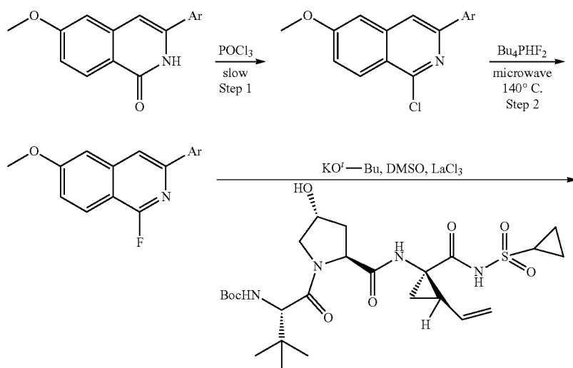
Scheme 4: (General Scheme)
