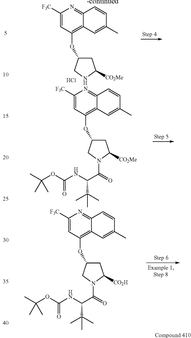
Compound 410
