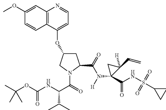
Compound 378
