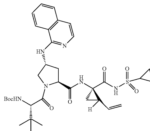
Compound 357
