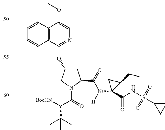
Compound 291
