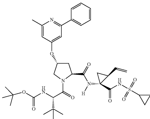
Compound 437
