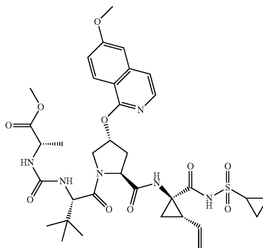
Compound 145
