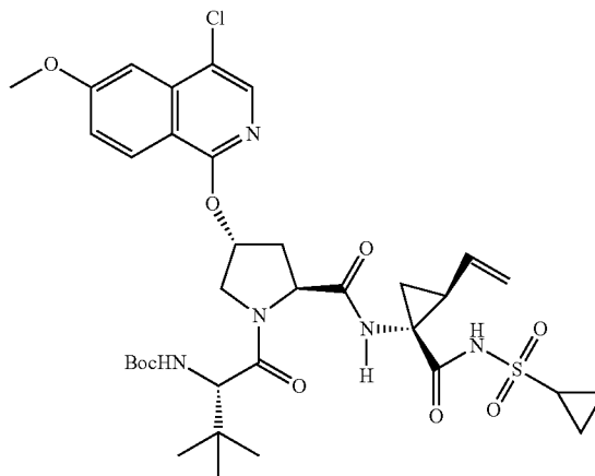
Compound 278
