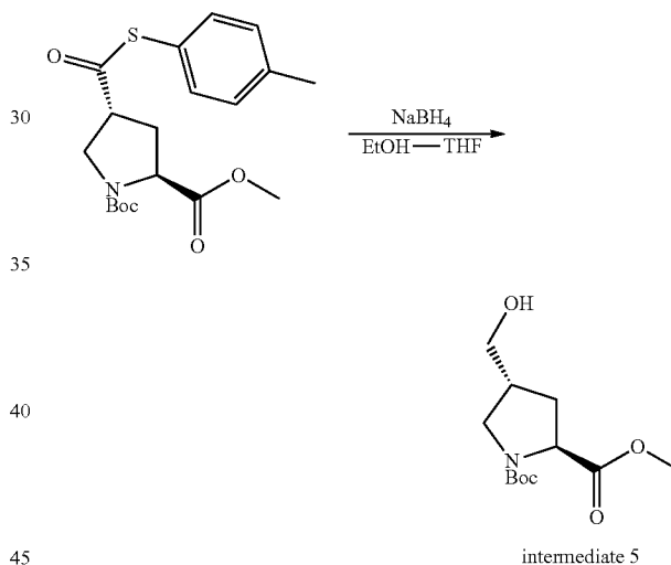
intermediate 5
