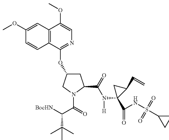
Compound 279
