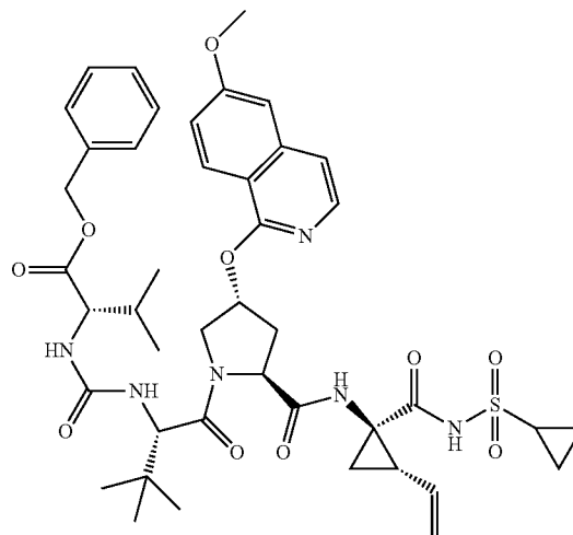
Compound 150
