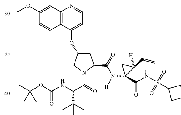
Compound 374
