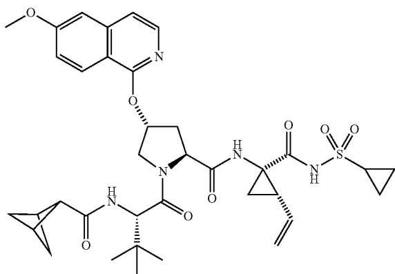
Compound 62
