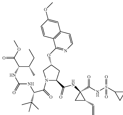
Compound 151
