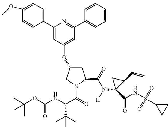
Compound 414
