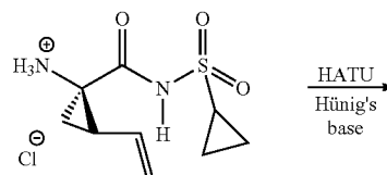
Example 180c
