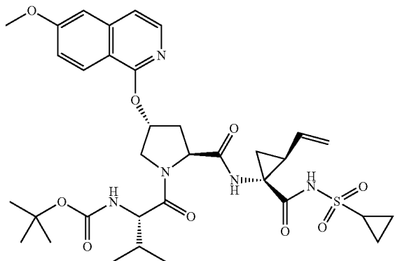
Compound 12
