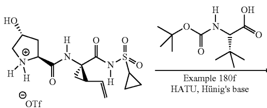
Example 184b
