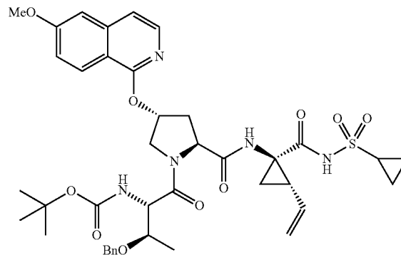
Compound 110
