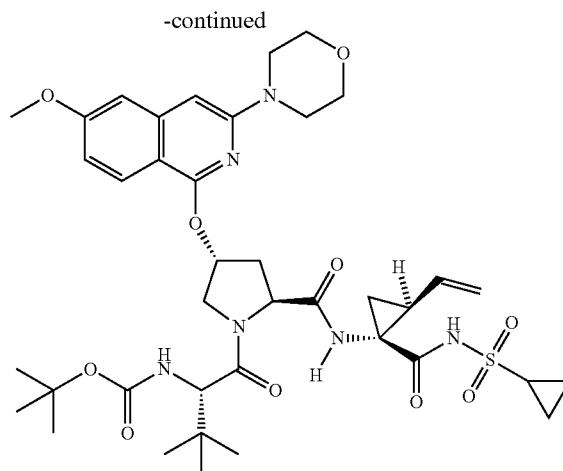
Compound 385
