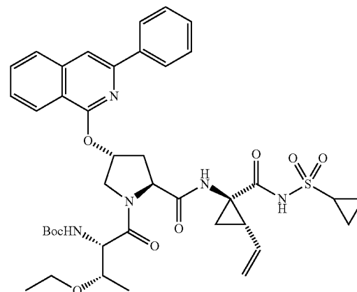
Compound 109
