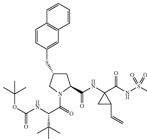
Compound 452
