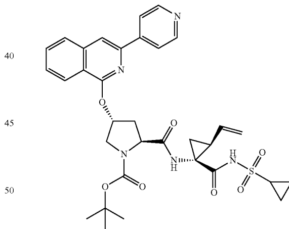
Compound 27
