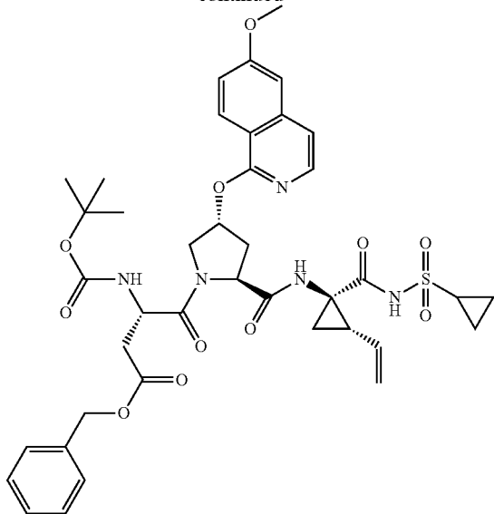
Compound 137
