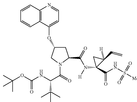
Compound 386
