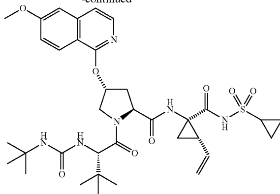
Compound 74
