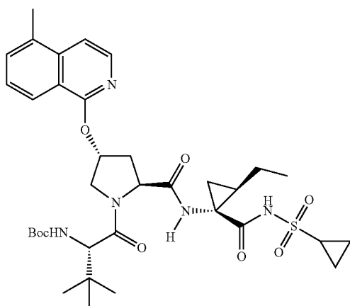
Compound 293
