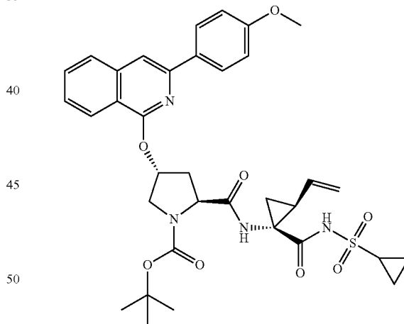
Compound 26
