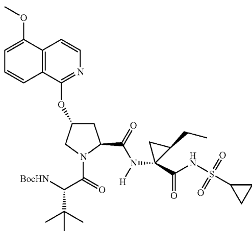
Compound 292
