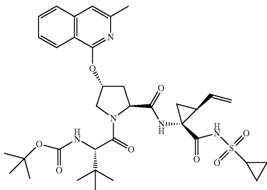
Compound 33
