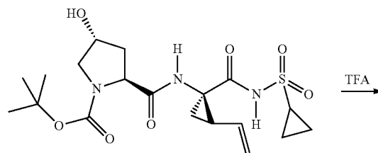
Example 184a
