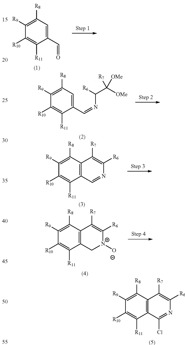
Scheme XII
