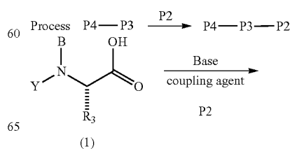
Scheme V
