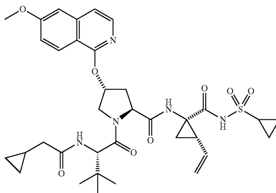
Compound 58
