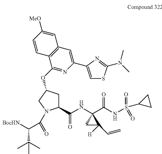
Compound 322
