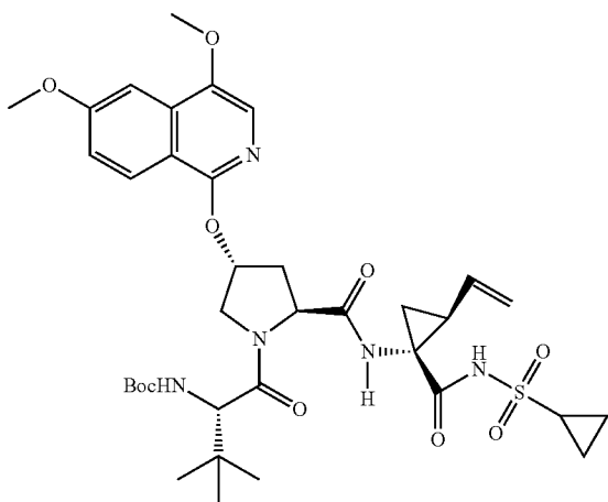
Compound 279
