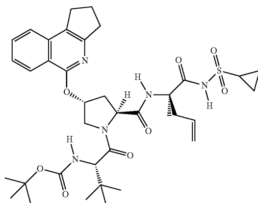
Example 215
