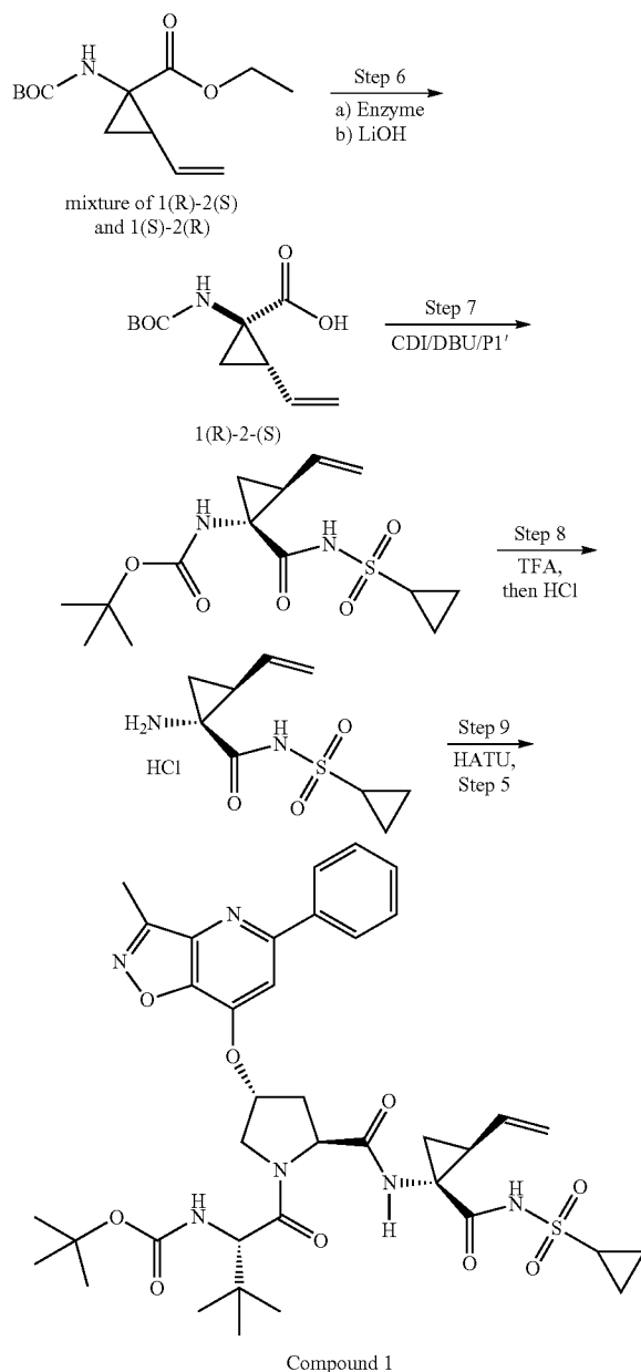
Scheme 3
