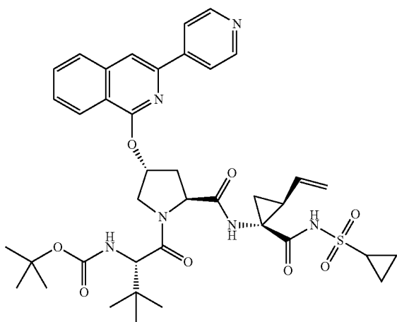
Compound 27
