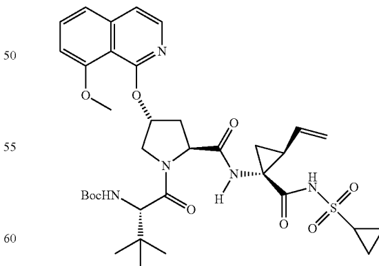
Compound 264
