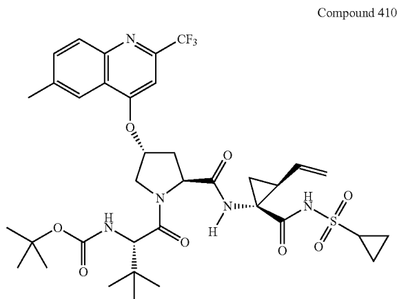
Compound 410
