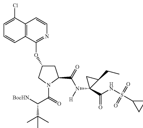
Compound 294
