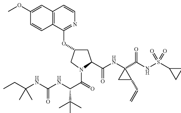
Compound 76
