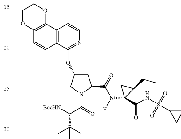
Compound 290
