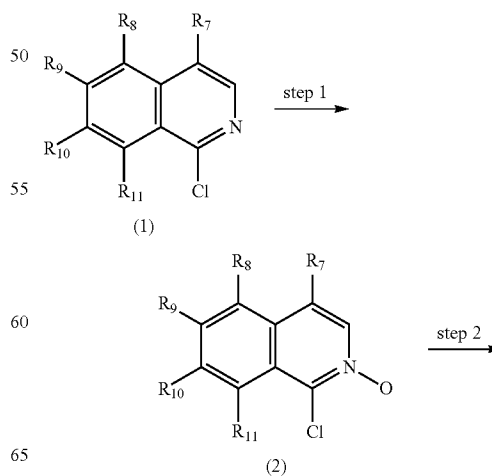
Scheme XVIII
