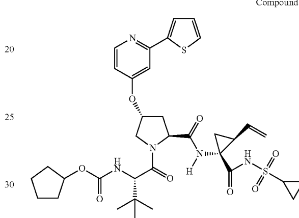
Compound 429
