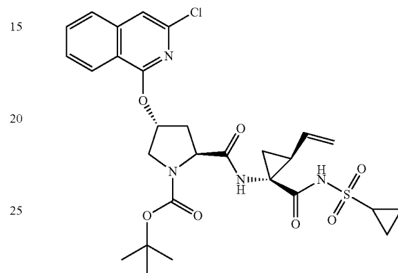
Compound 24
