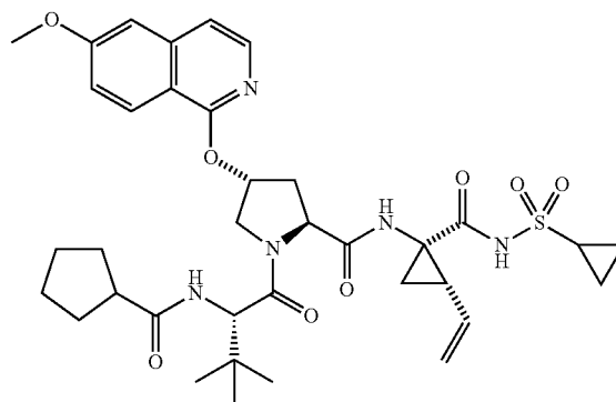
Compound 56
