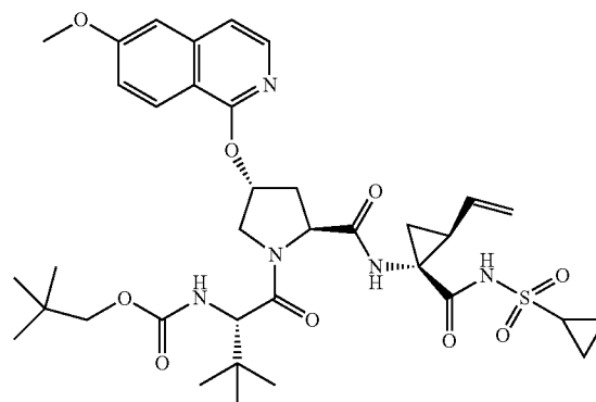
Compound 18
