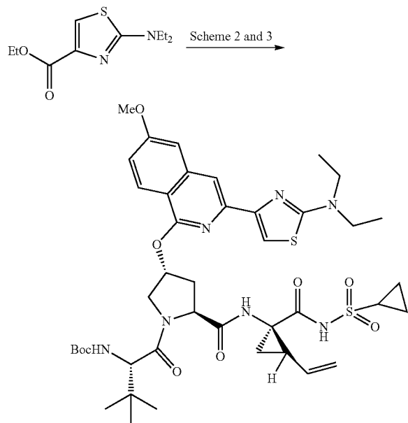
Compound 321
