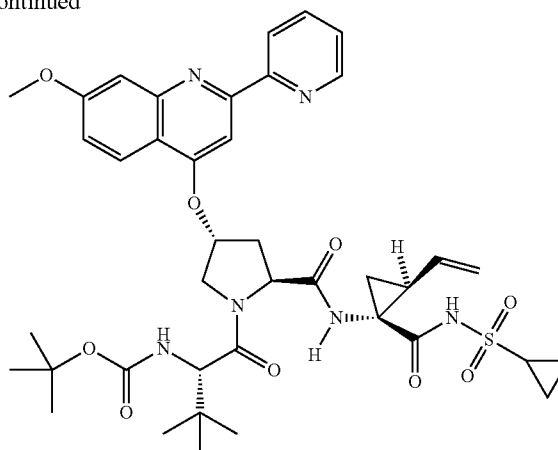
Compound 379
