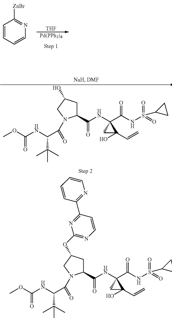
Compound 336
