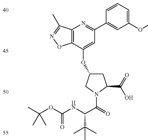
Compound 5
