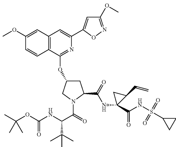
Compound 38
