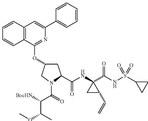
Compound 108
