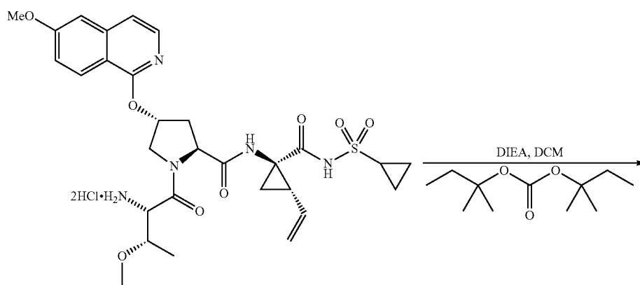
Compound 100
