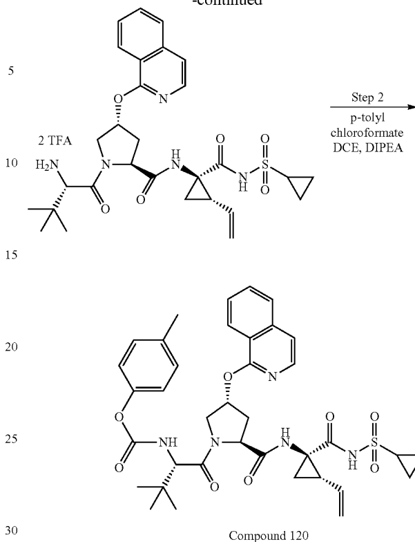
Compound 120
