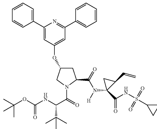
Compound 415
