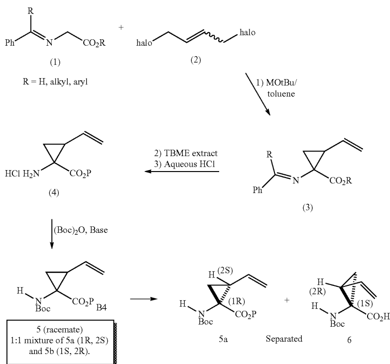
Scheme VIII
