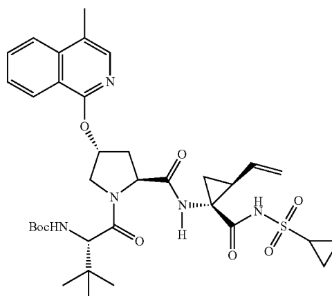
Compound 250
