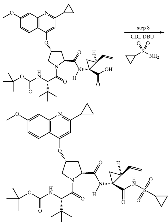
Compound 373
