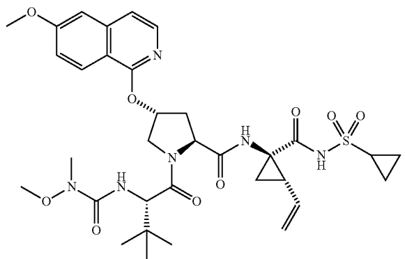
Compound 78
