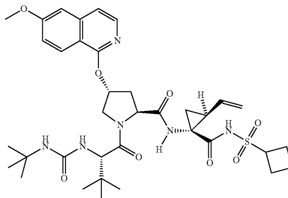
Compound 383
