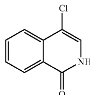
Compound 280 10
