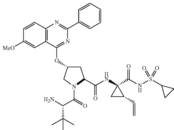
Compound 50
