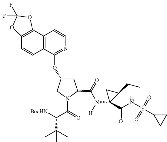
Compound 289
