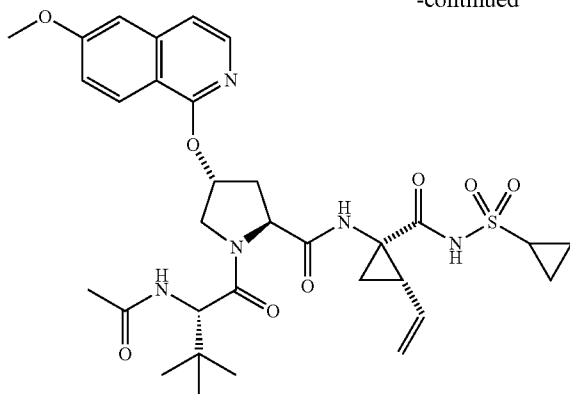
Compound 55
