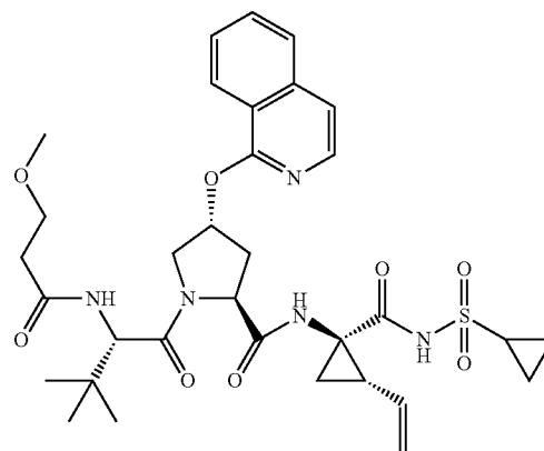
Compound 132
