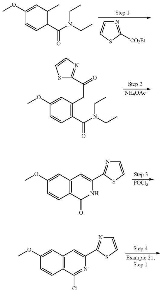
Scheme 1
