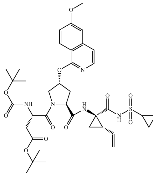
Compound 139
