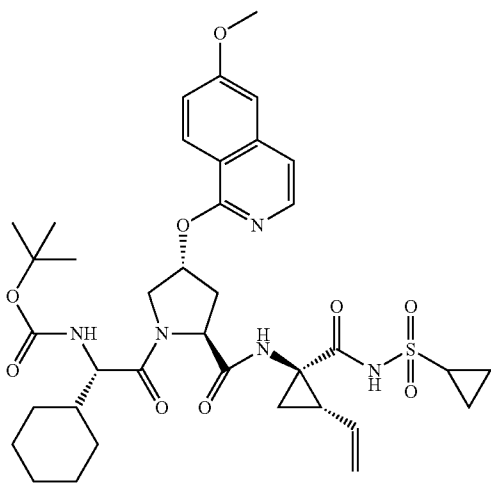
Compound 143
