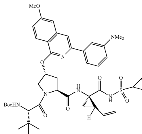
Compound 330
