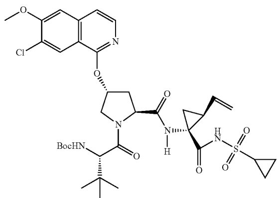
Compound 273 45
