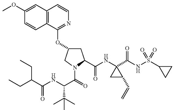
Compound 57
