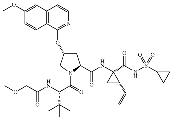
Compound 59
