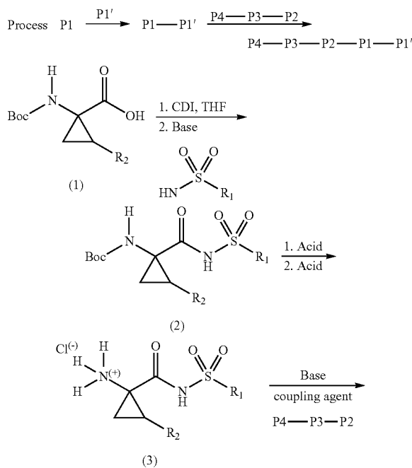
Scheme III
