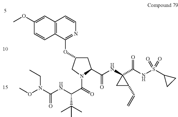
Compound 79
