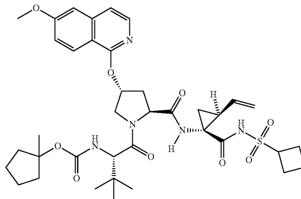
Compound 384
