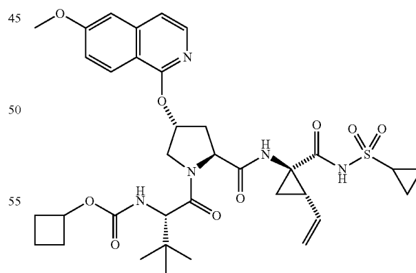
Compound 71
