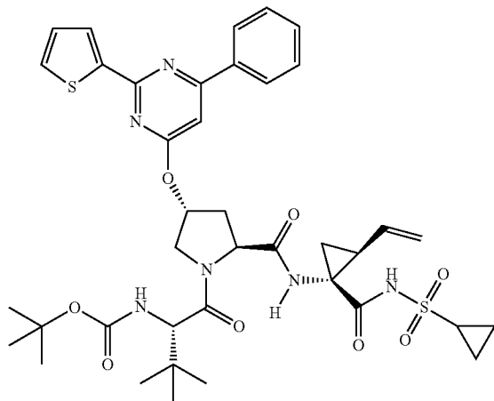
Compound 413
