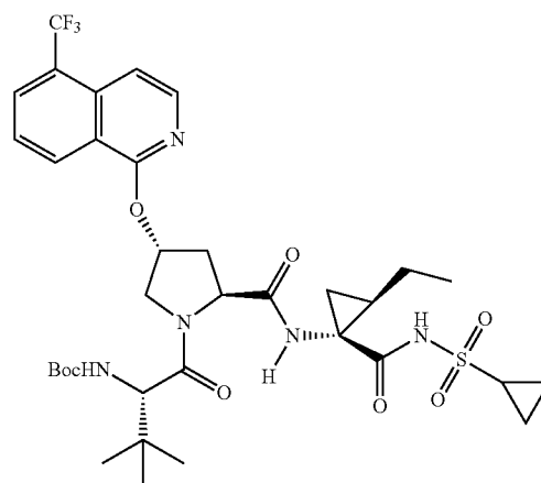
Compound 295
