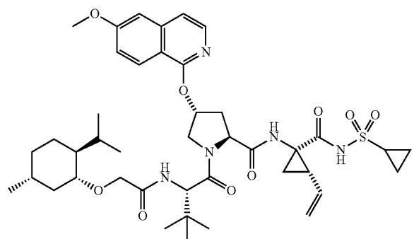
Compound 61
