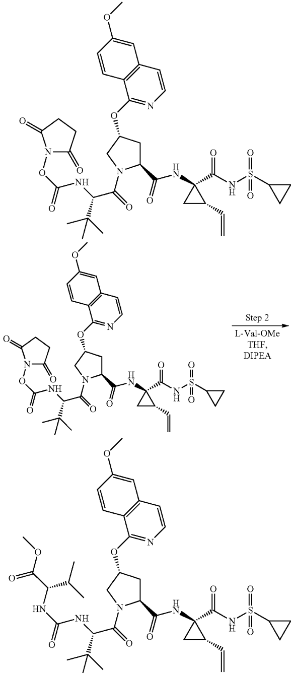
Compound 141
