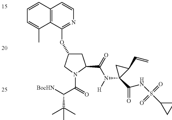
Compound 263
