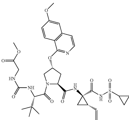
Compound 144
