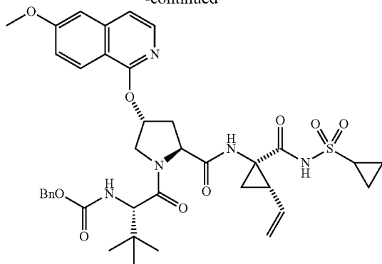
Compound 64
