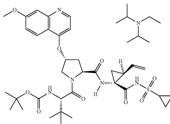
Compound 375
