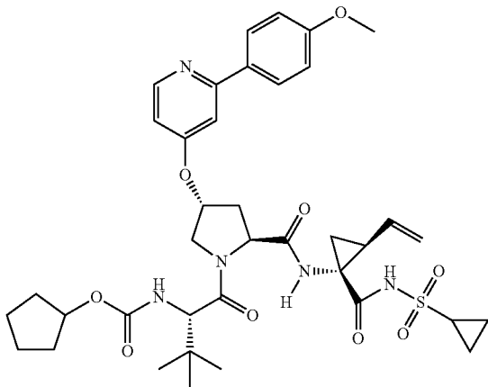
Compound 428
