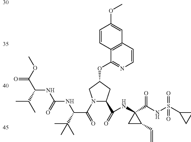
Compound 142
