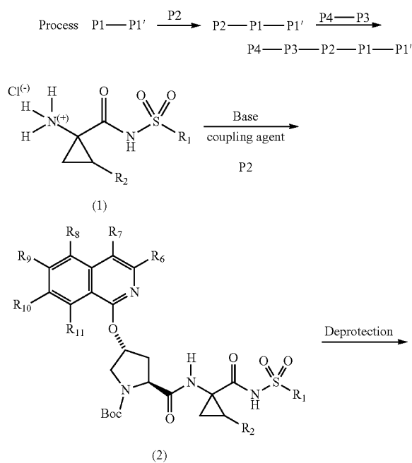
Scheme IV
