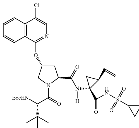
Compound 281
