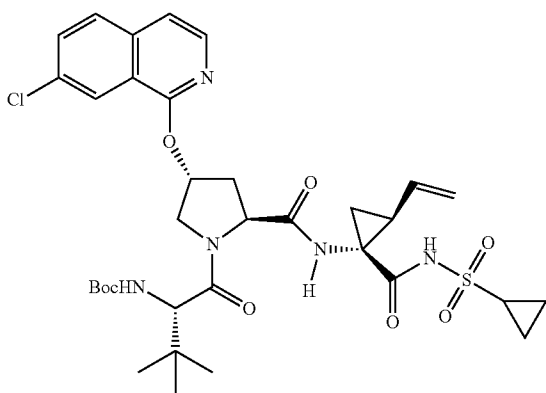
Compound 258
