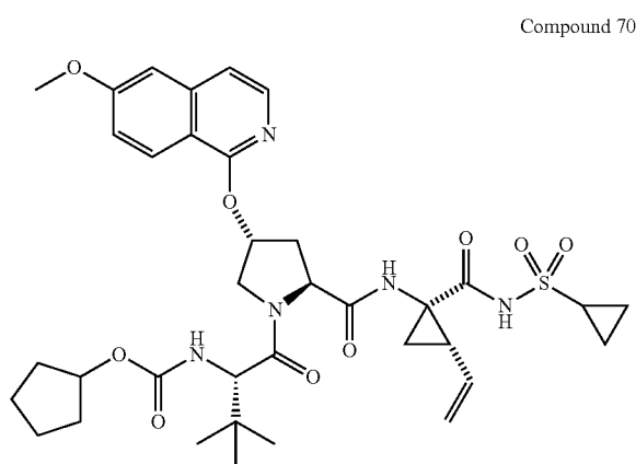
Compound 70
