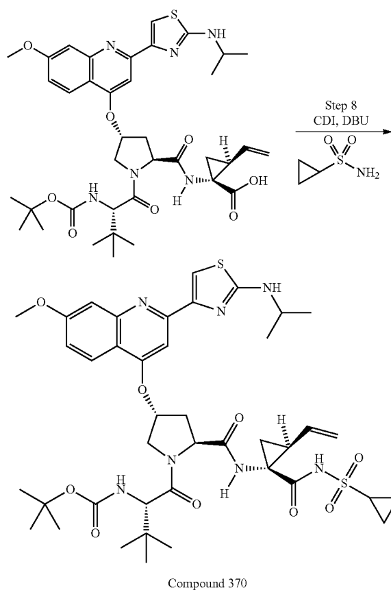
Scheme 3
