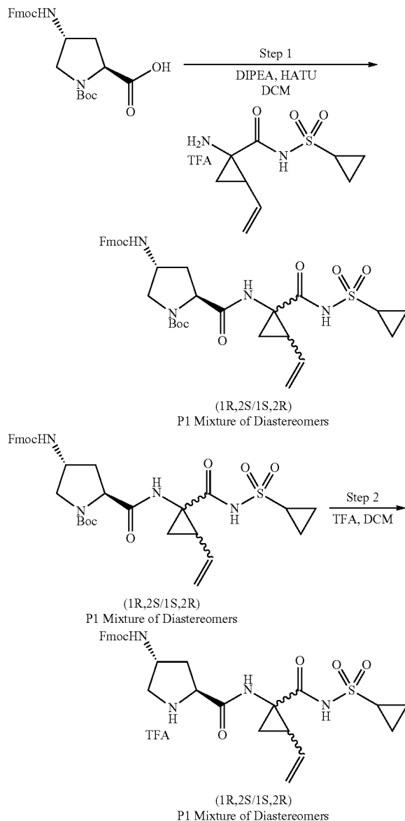
Scheme 1
