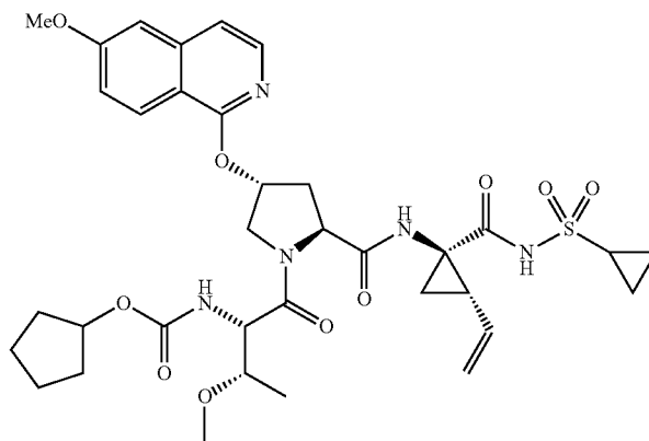
Compound 104
