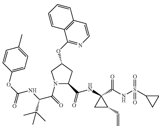
Compound 120
