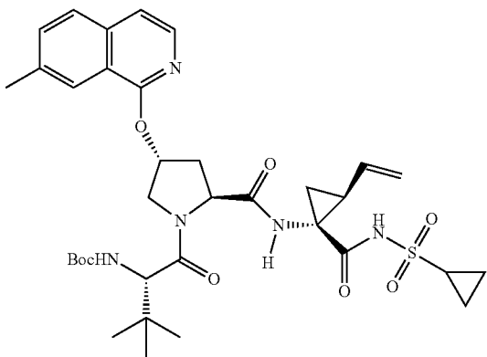
Compound 259
