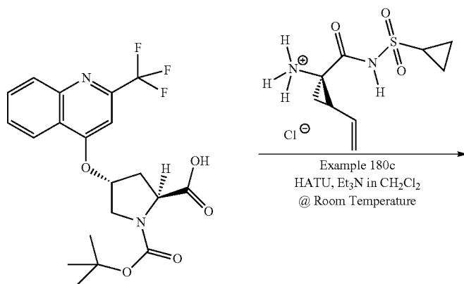
Example 180b
