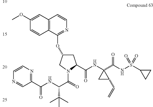
Compound 63
