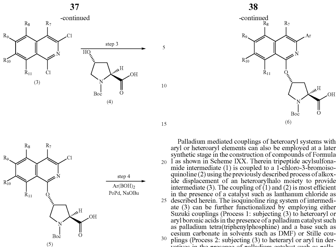
Scheme IXX
