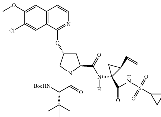
Compound 273 50
