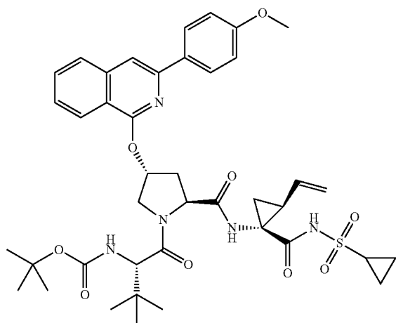
Compound 26
