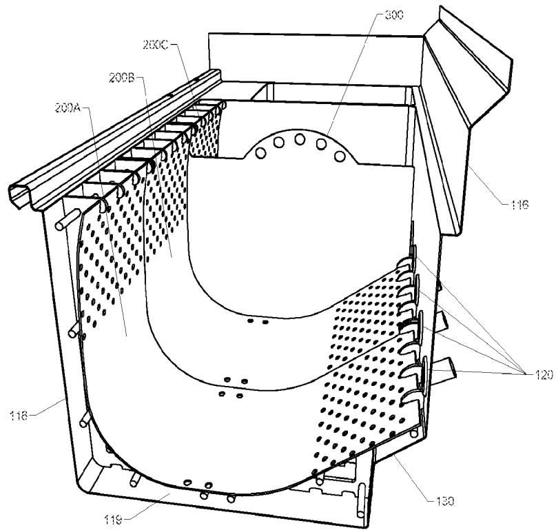
TRANSVERSE SECTION
