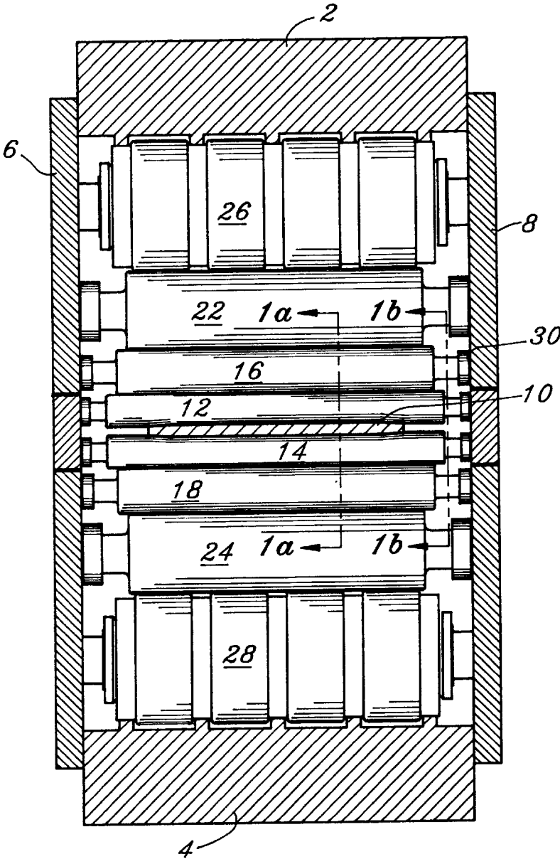
Fig. 1 (Prior Art)
