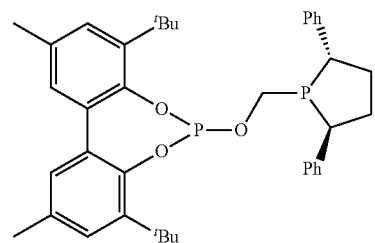
(tropos,R,R)-3
