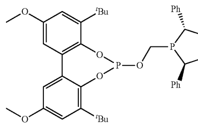
(tropos,R,R)-2
