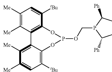
(atropos,R,R,R)-1
