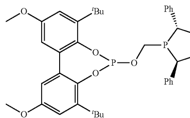
(tropos,trans)-2
