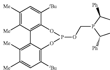
(atropos,R,R,R)-1/(atropos,S,S,S)-1 mixture
