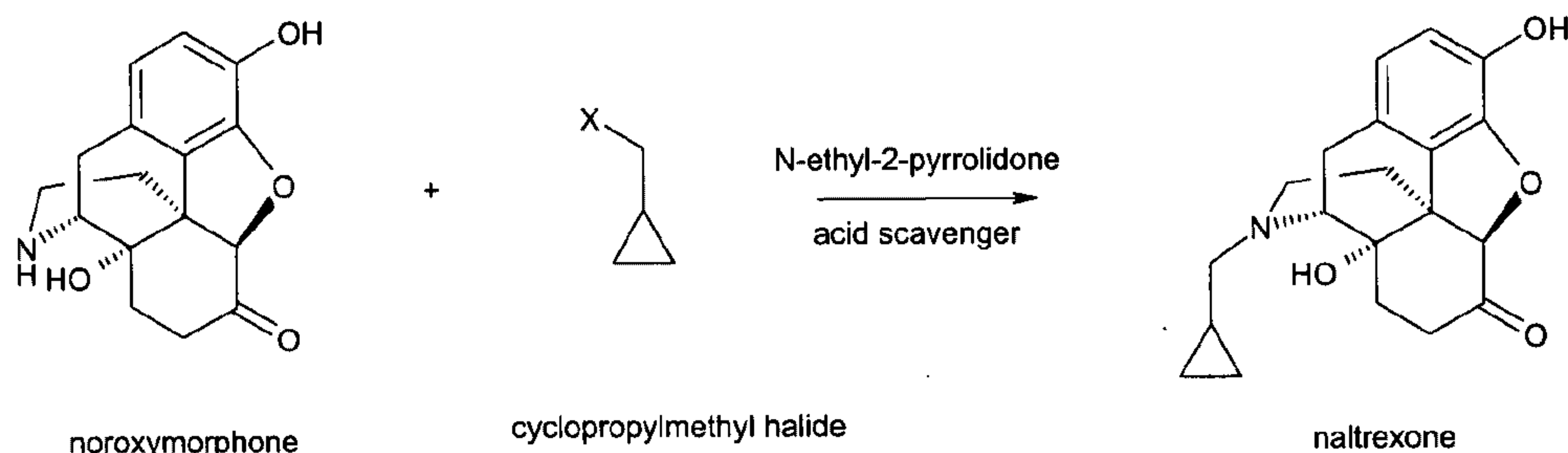
Scheme 1
