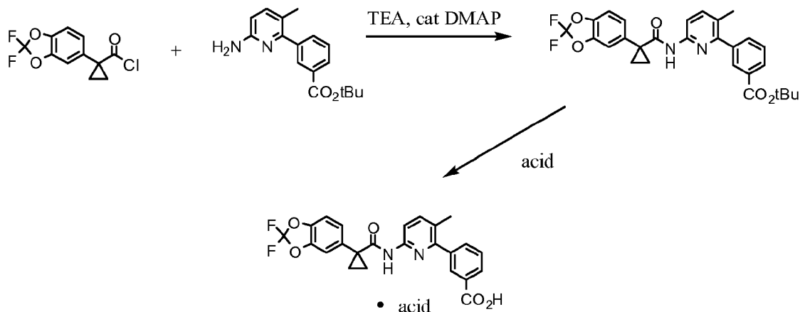
Scheme 3. Formation of an acid salt of 3-(6-(1-(2,2-difluorobenzo[d][1,3]dioxol-5-yl) cyclopropanecarboxamido)-3-methylpyridin-2-yl)benzoic acid.
