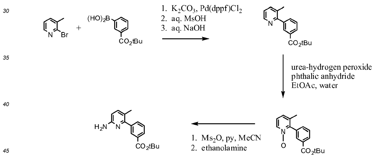
Scheme 2. Synthesis of the amine moiety.
