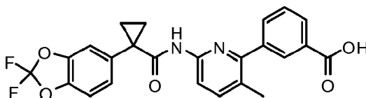
Compound 1.
