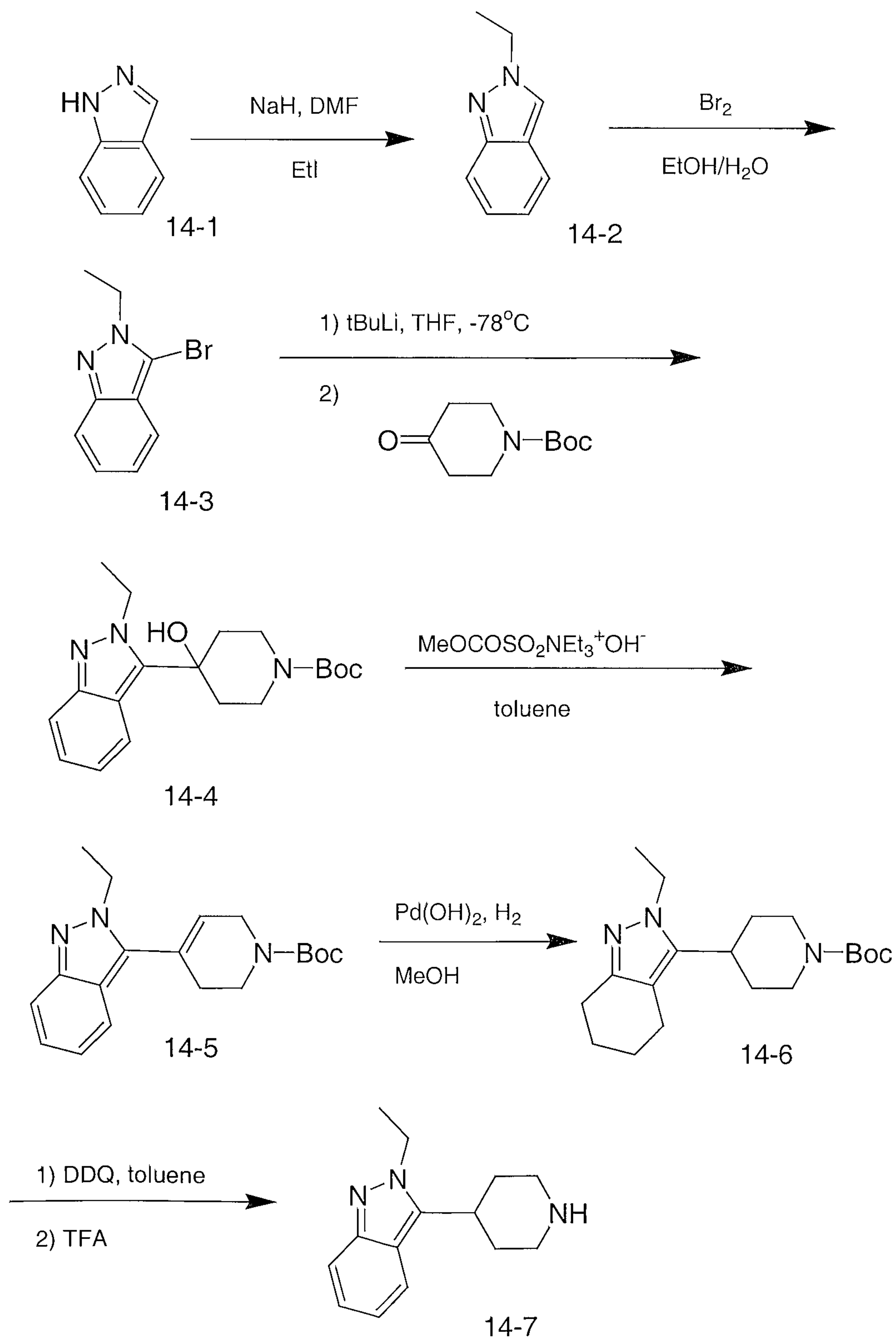
SCHEME 14
