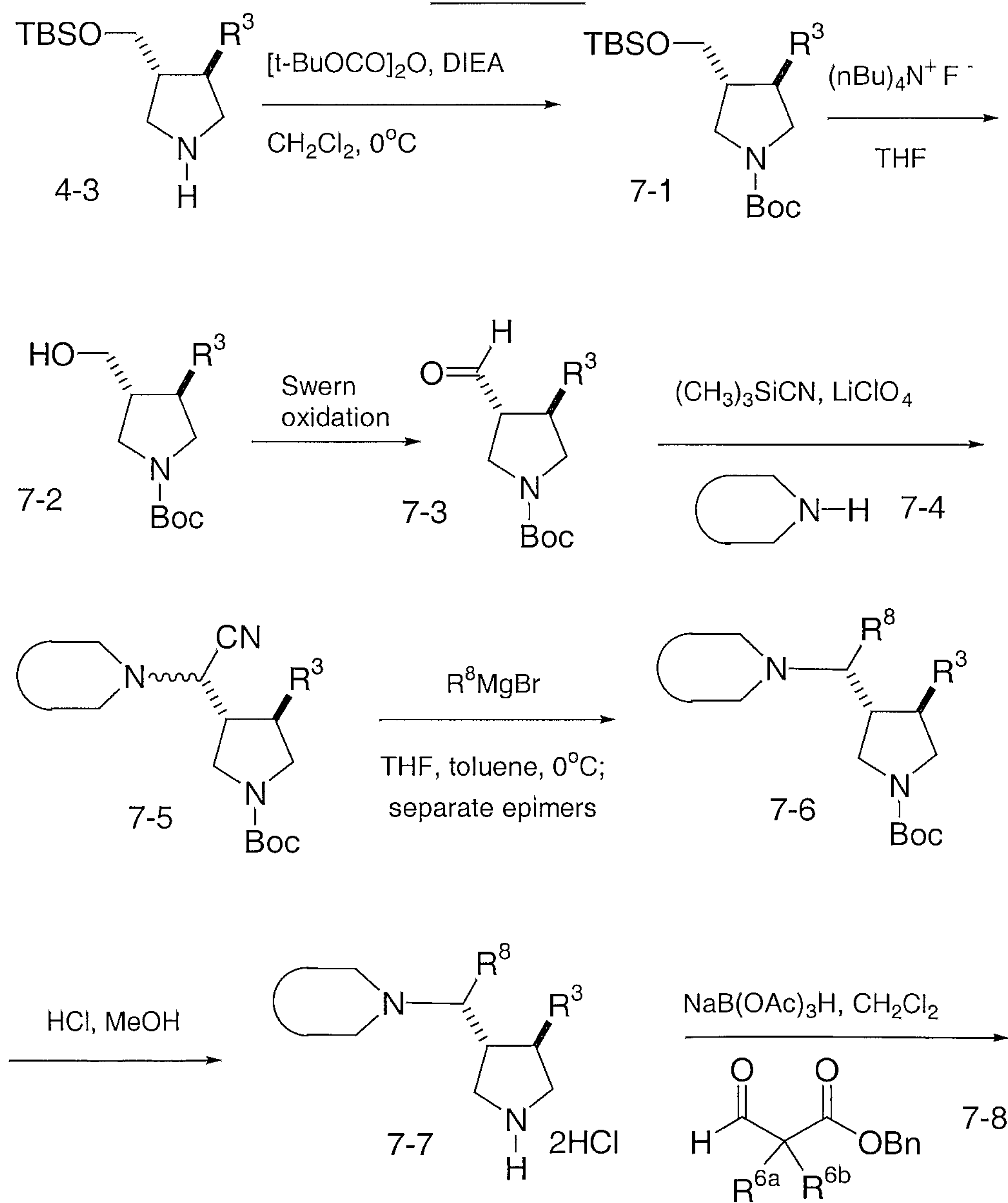
SCHEME 7
