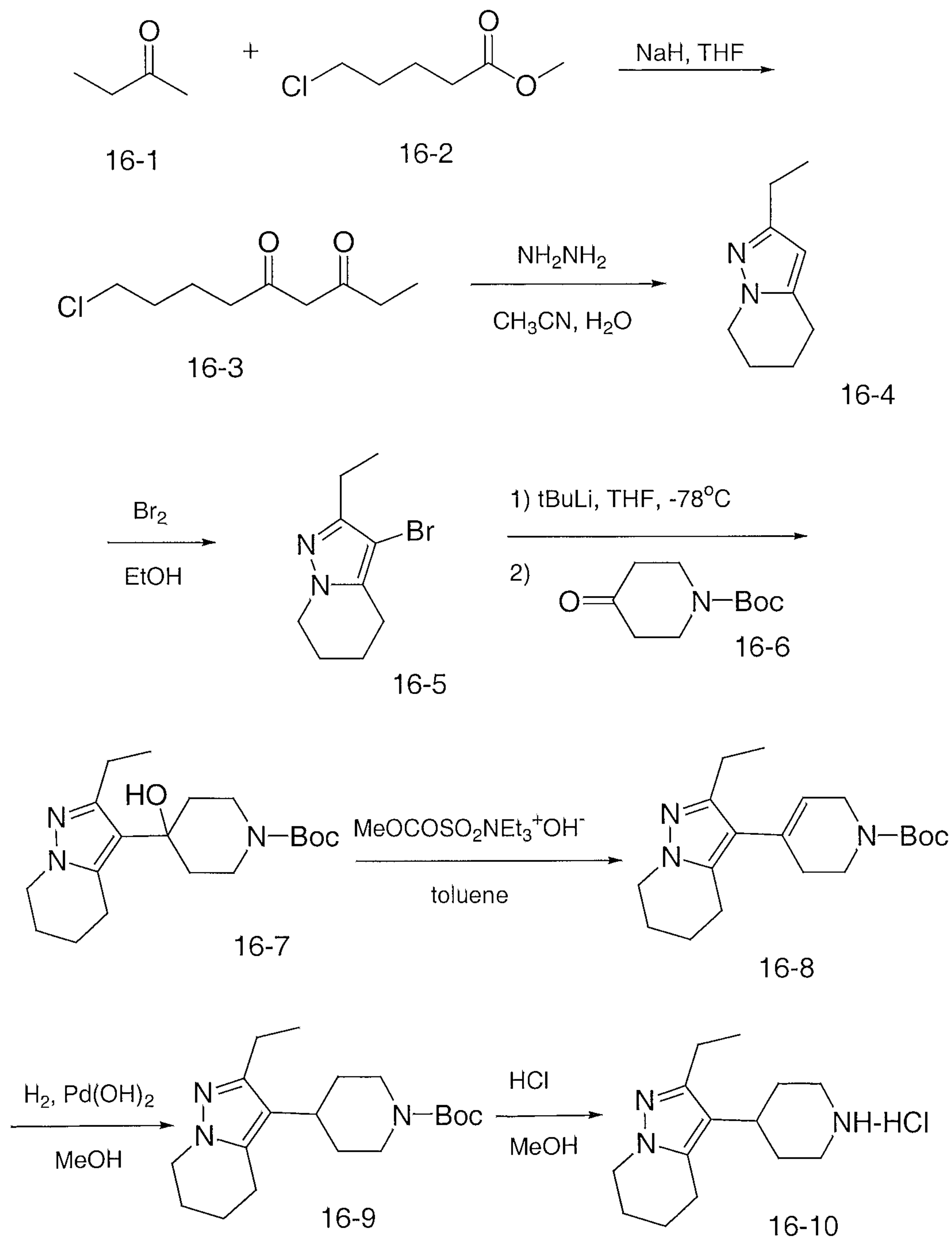
SCHEME 16
