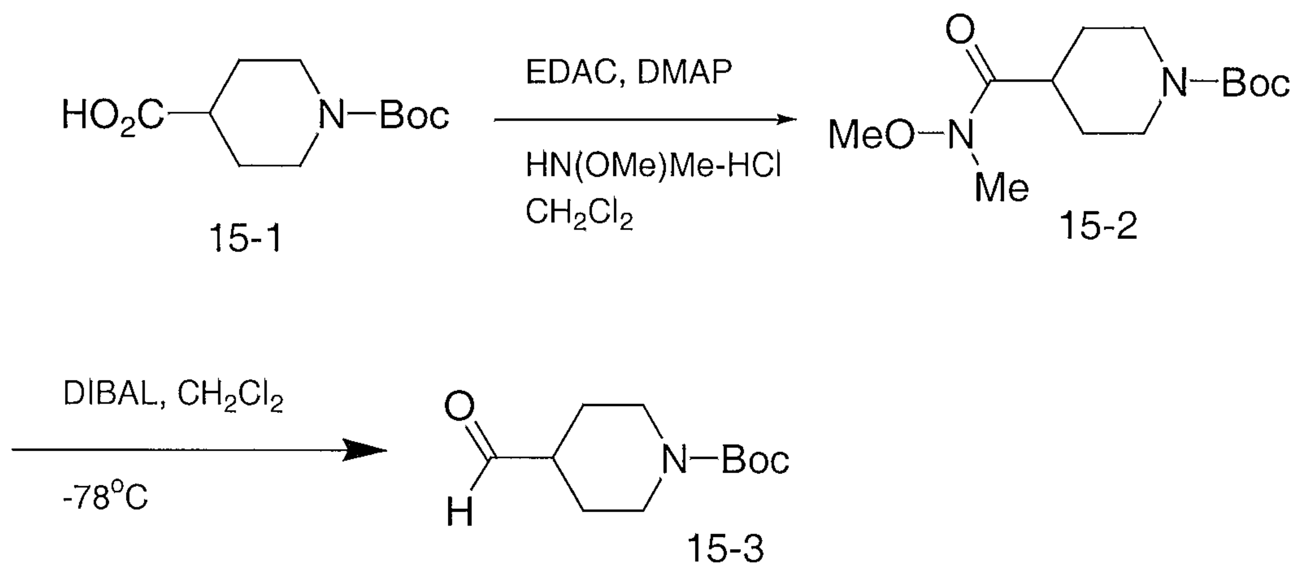
SCHEME 15
