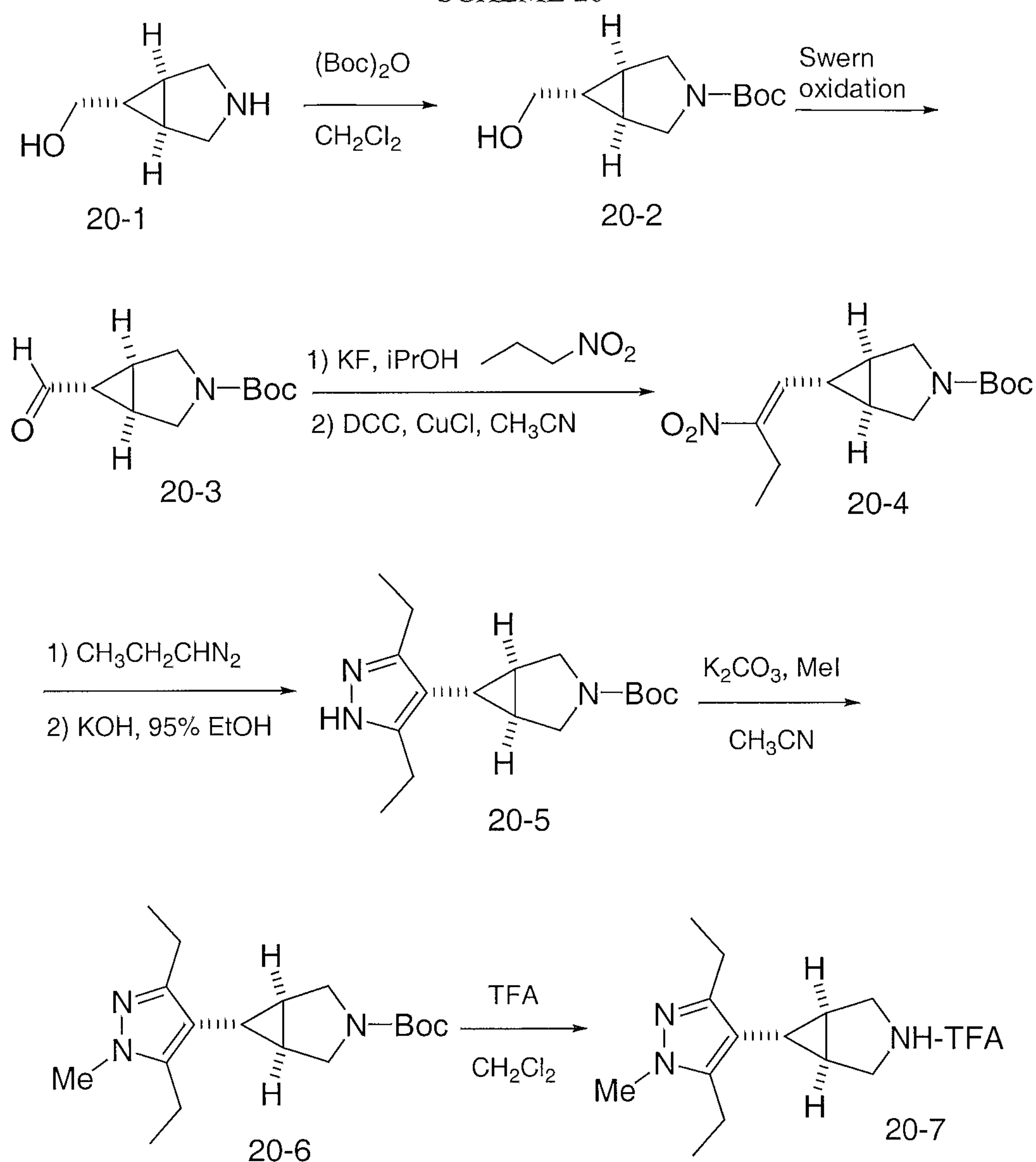
SCHEME 20
